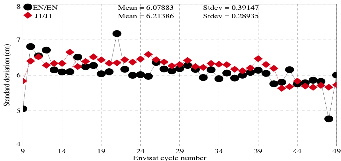
Std dev. of crossover points, |\text{Latitude}| < 50^\circ , Bathy < -1000\text{m} , Var < 20\text{cm}
