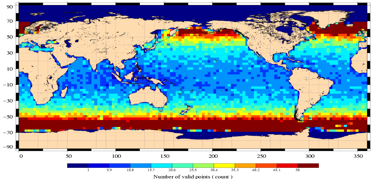
Number of Jason/Envisat 10 days cross-over points Cycle 054 (18/12/2006 – 22/01/2007)
