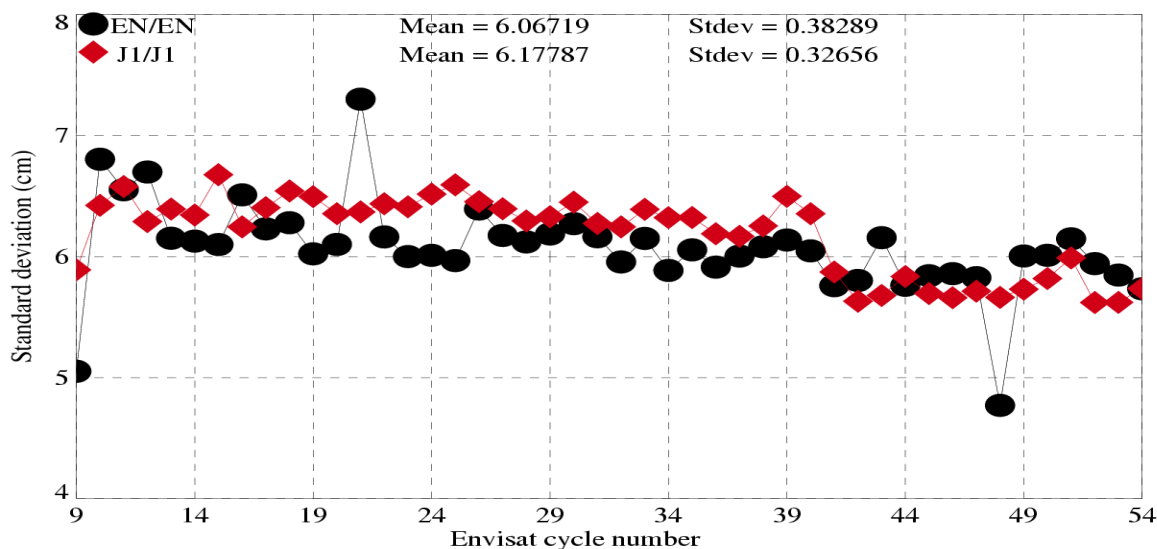
Std dev. of crossover points, |Latitude|<50°, Bathy<-1000m, Var<20cm
