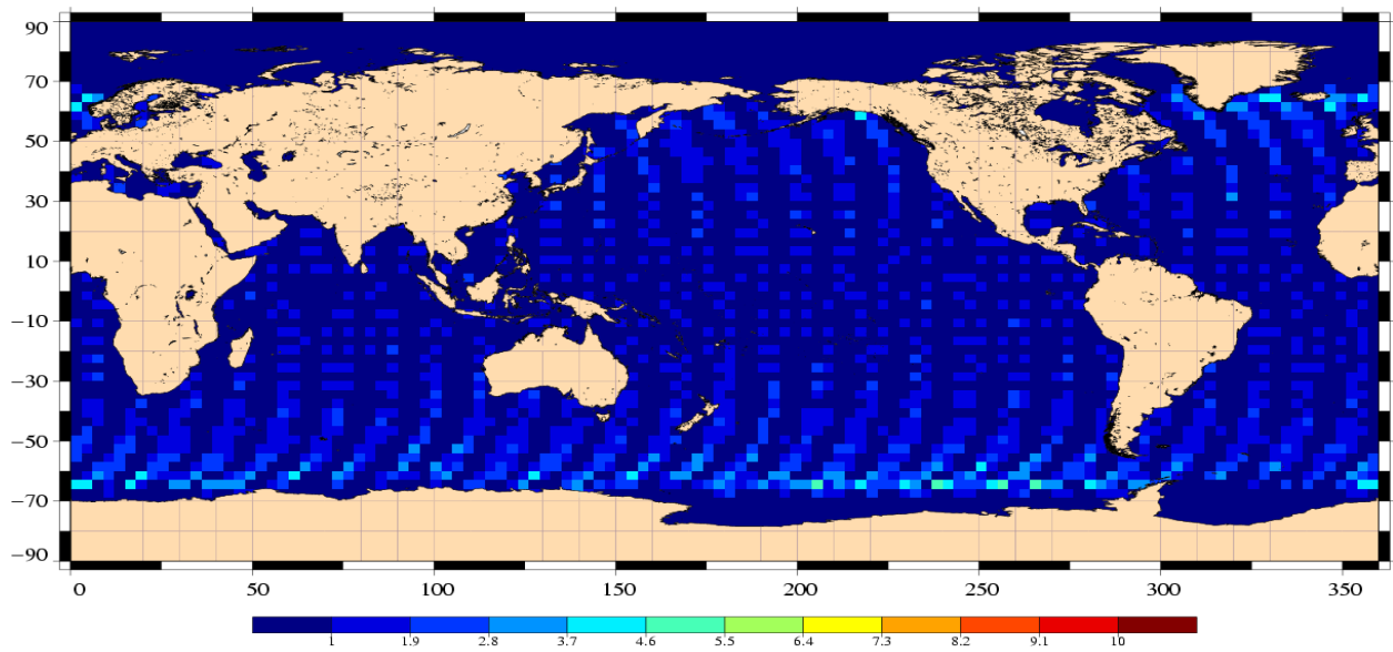
Number of Jason/Envisat 10 days cross-over points Cycle 054 (18/12/2006 – 22/01/2007)
