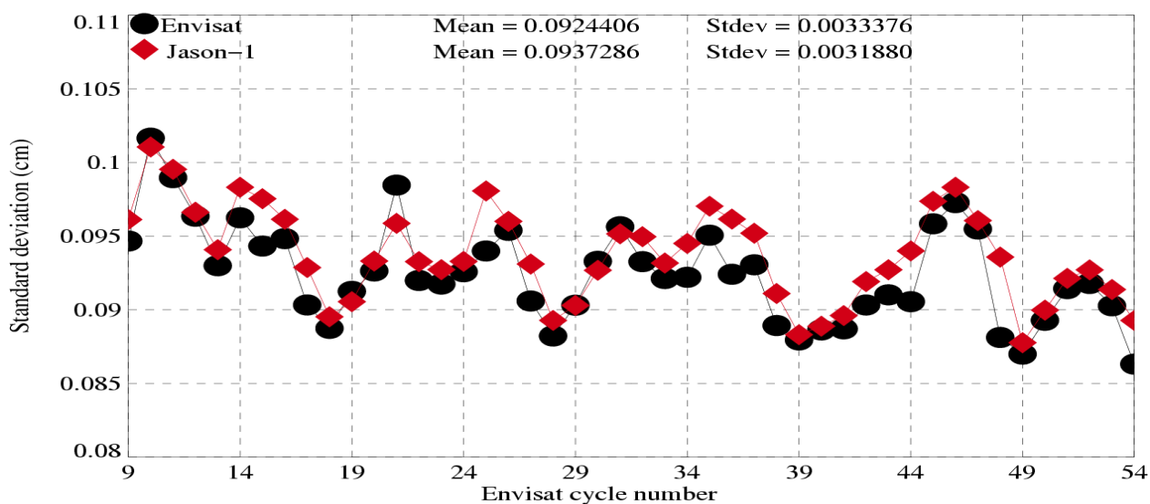
Std dev. of SSH–MSS, |\text{Latitude}| < 50^\circ , Bathy < -1000\text{m} , Var < 20\text{cm}
