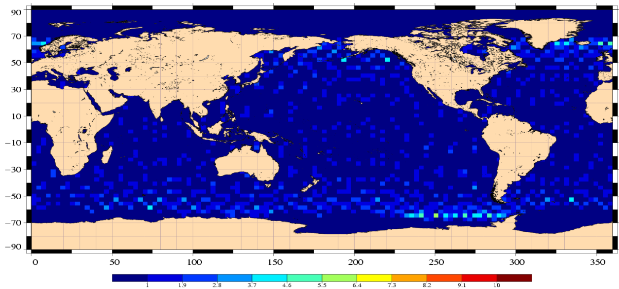
Number of Jason/Envisat 10 days cross-over points Cycle 063 (29/10/2007 – 03/12/2007)
