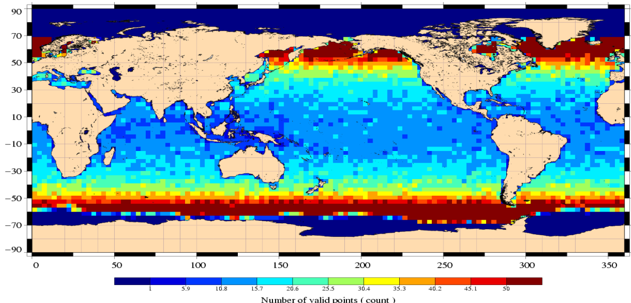
Number of Jason/Envisat 10 days cross-over points Cycle 063 (29/10/2007 – 03/12/2007)
