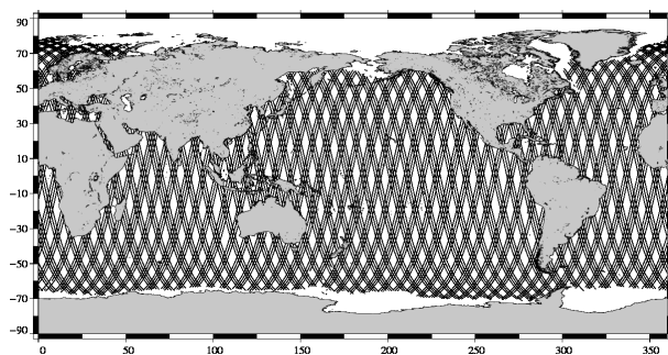
ENVISAT 10-day coverage for Jason-2 cycle 29
