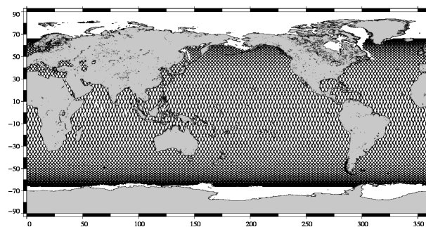
JASON 2 10-day coverage for Jason-2 cycle 29
