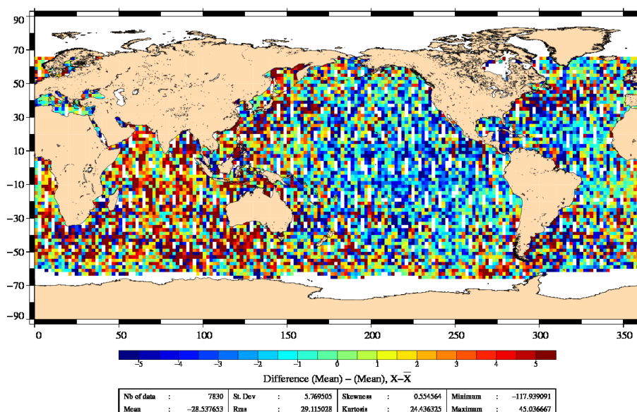
Differences of SLA before orbit error correction J2 – EN (14/06/2009 to 24/06/2009)
