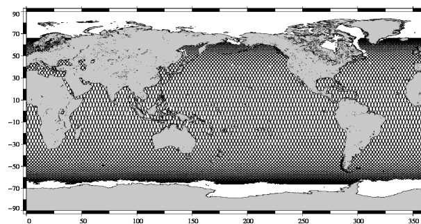
JASON 2 10-day coverage for Jason-2 cycle 32
