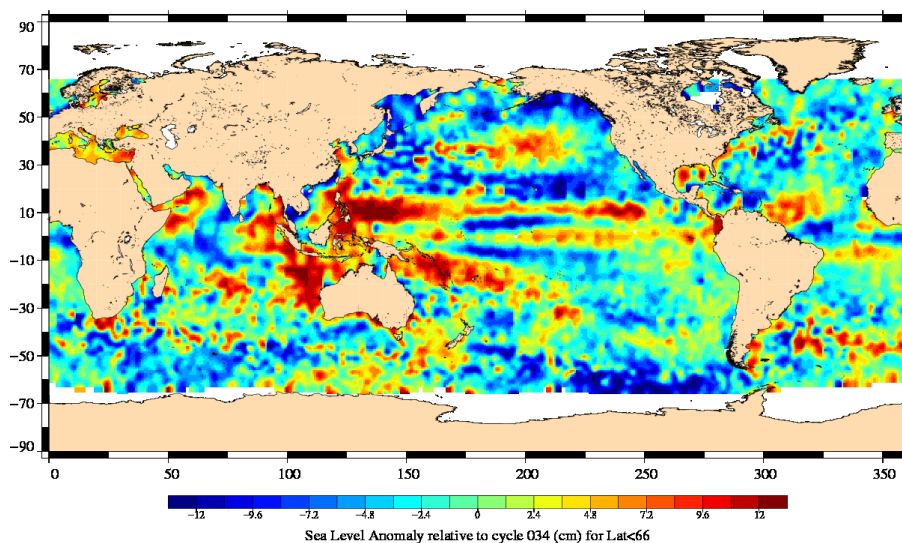
Variability relative to MSS (cm) Cycle 035 EN (14/06/2009 to 24/06/2009)
