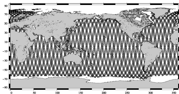
ENVISAT 10-day coverage for Jason-2 cycle 32
