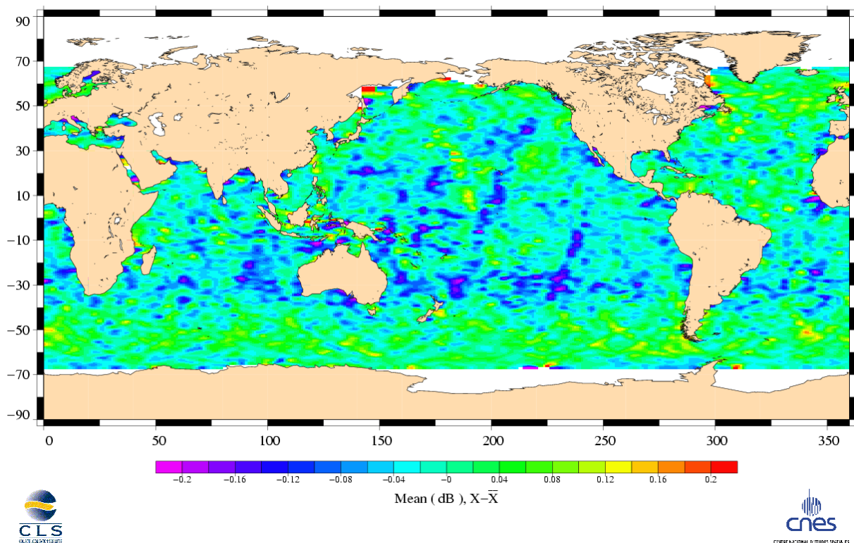
Ku SIGMA0 differences Topex (Cycle 344) – Jason (Cycle 001)
