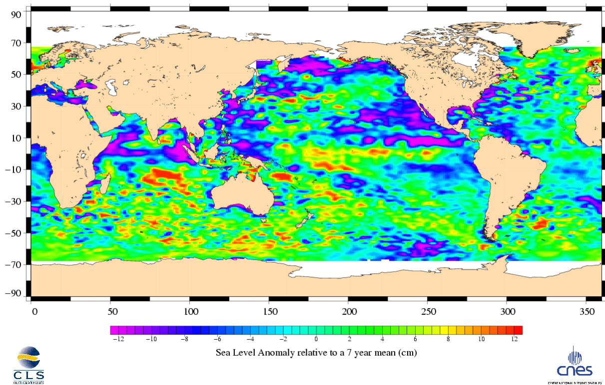
Jason-1 Cycle 001 15/01/2002 – 24/01/2002
