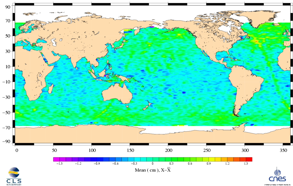
Altimeter ionospheric correction differences Topex (Cycle 344) – Jason (Cycle 001)
