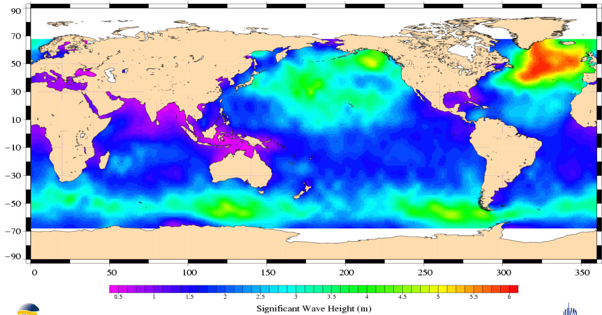
Jason-1 Cycle 001 15/01/2002 – 24/01/2002
