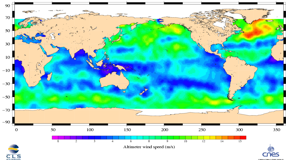
Jason-1 Cycle 001 15/01/2002 – 24/01/2002
