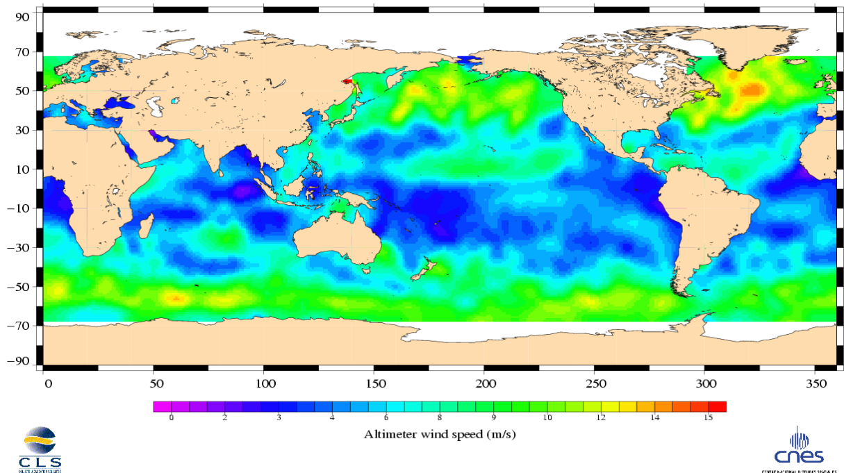
Jason-1 Cycle 003 04/02/2002 – 13/02/2002
