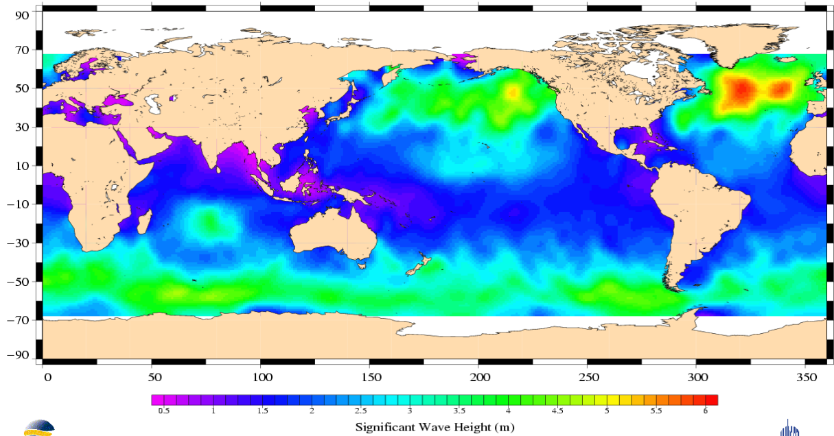
Jason-1 Cycle 003 04/02/2002 – 13/02/2002
