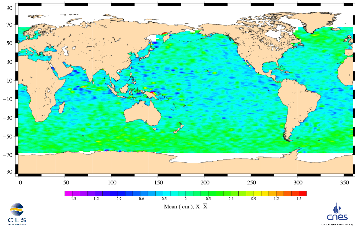
Altimeter ionospheric correction differences Topex (Cycle 352) – Jason (Cycle 009)
