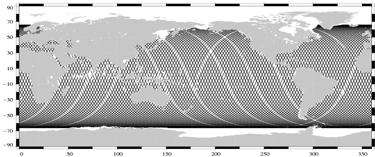
Valid data Jason-1 Cycle 009 (04/04/2002 / 14/04/2002)
