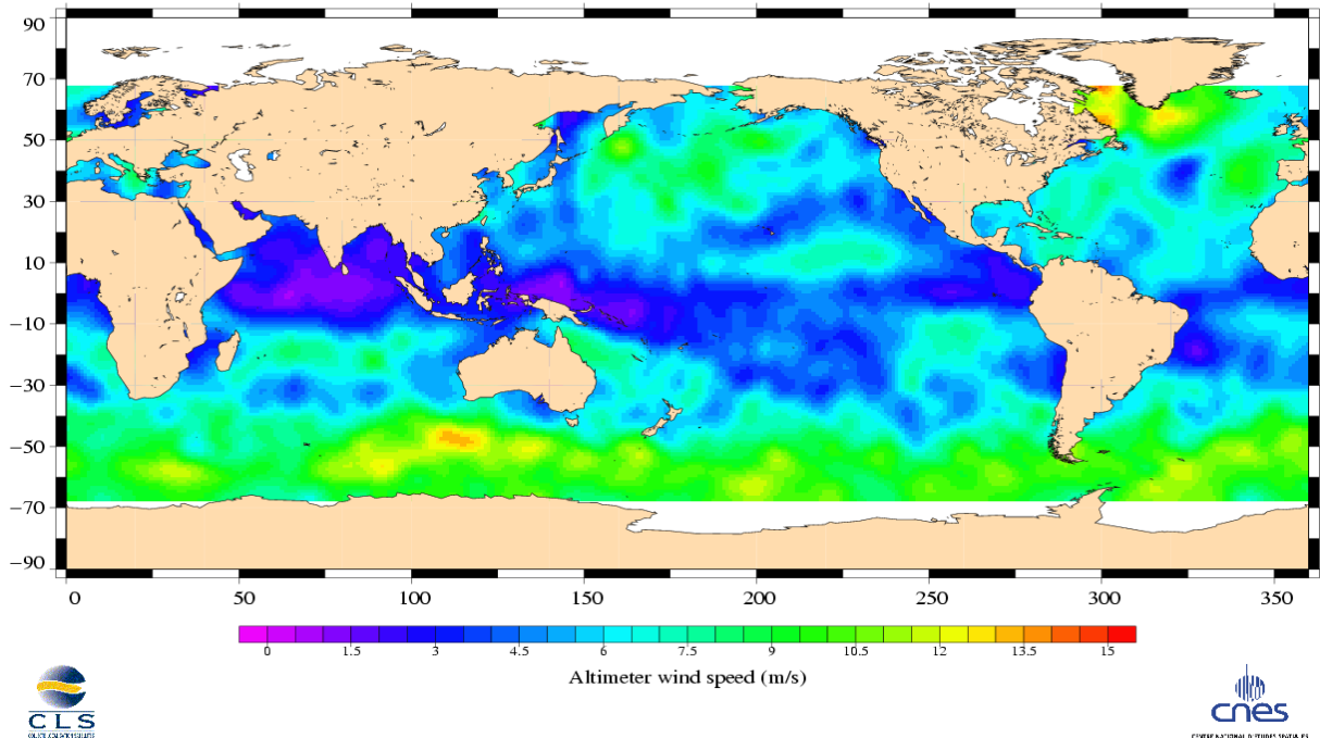
Jason-1 Cycle 009 04/04/2002 - 14/04/2002
