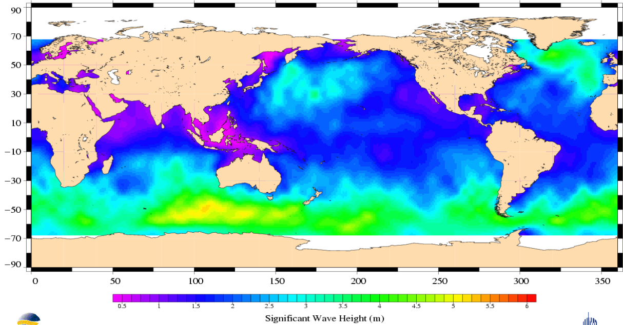
Jason-1 Cycle 009 04/04/2002 - 14/04/2002
