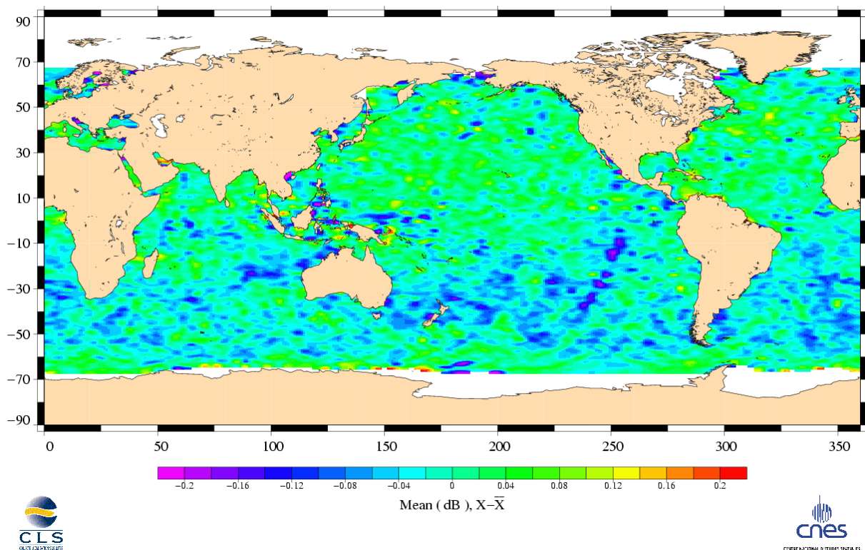
Ku SIGMA0 differences Topex (Cycle 355) – Jason (Cycle 012)
