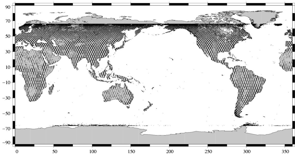
Missing measurements Jason-1 Cycle 012 (04/05/2002 / 14/05/2002)
