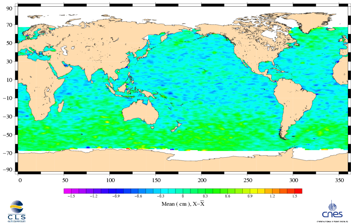
Altimeter ionospheric correction differences Topex (Cycle 355) – Jason (Cycle 012)
