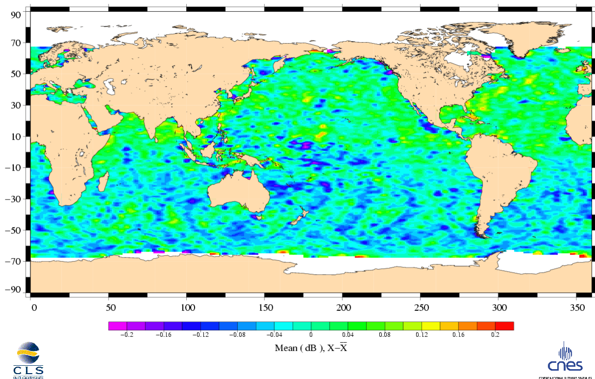
Ku SIGMA0 differences Topex (Cycle 356) – Jason (Cycle 013)
