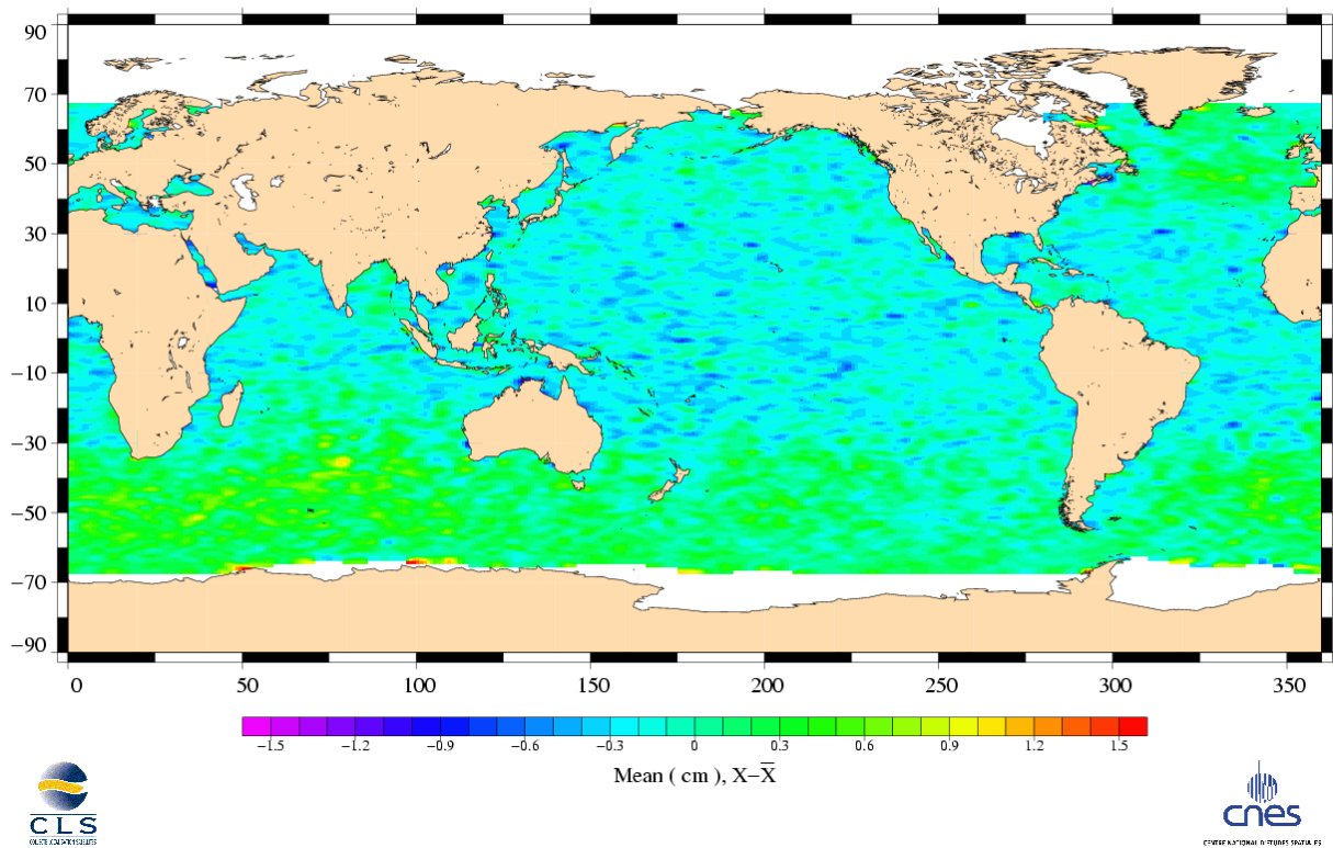
Altimeter ionospheric correction differences Topex (Cycle 356) – Jason (Cycle 013)
