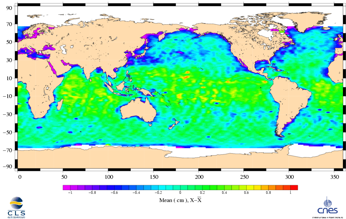
Radiometer correction differences Topex (Cycle 356) – Jason (Cycle 013)
