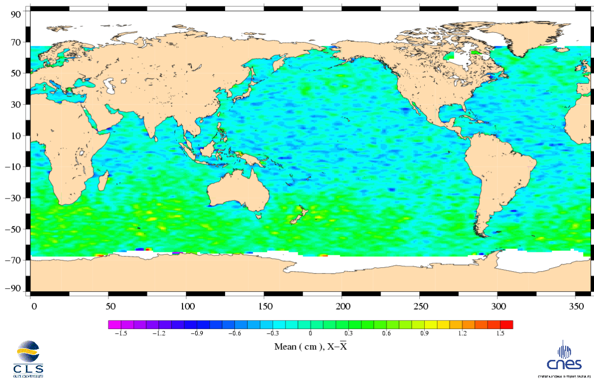
Altimeter ionospheric correction differences Topex (Cycle 357) – Jason (Cycle 014)
