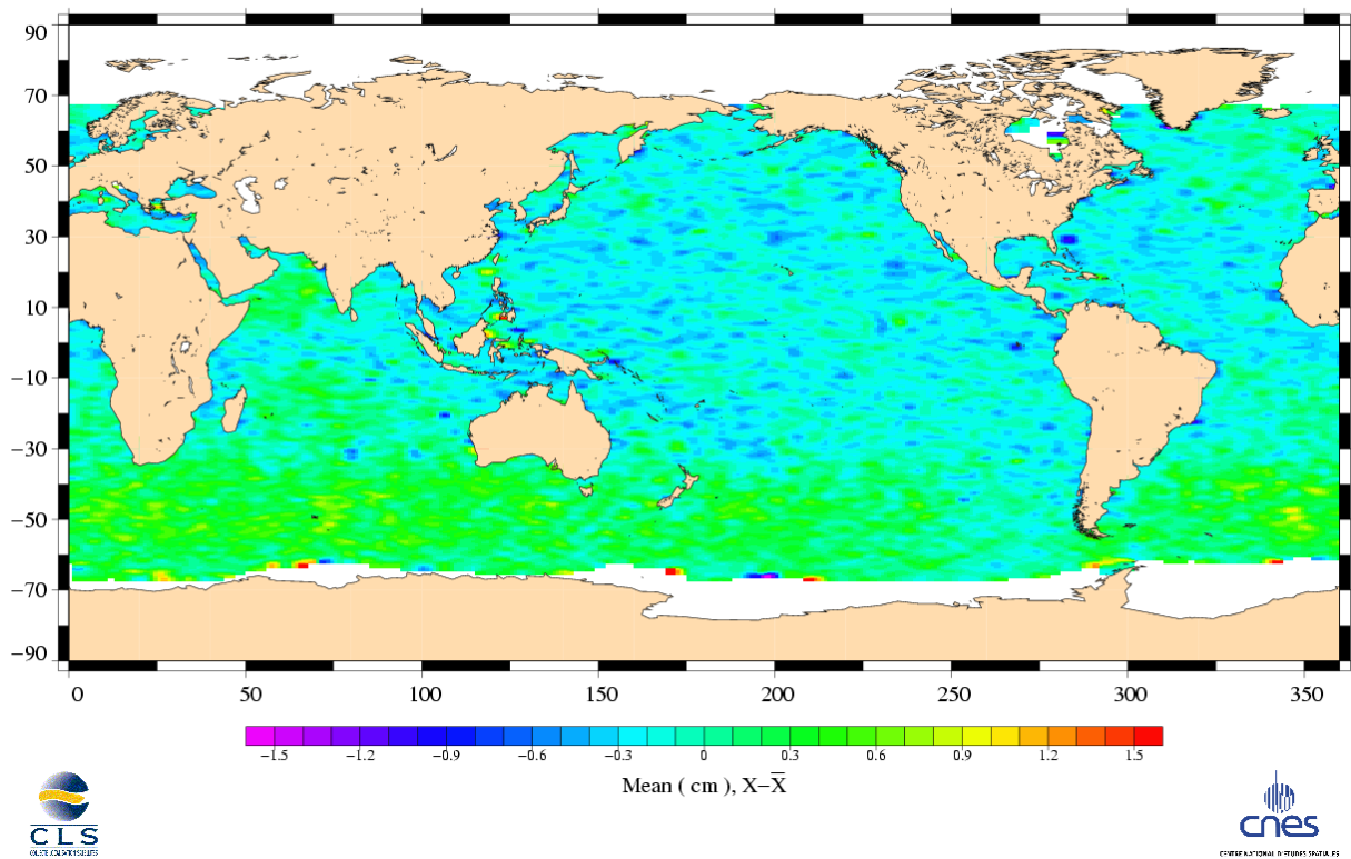
Altimeter ionospheric correction differences Topex (Cycle 359) – Jason (Cycle 016)
