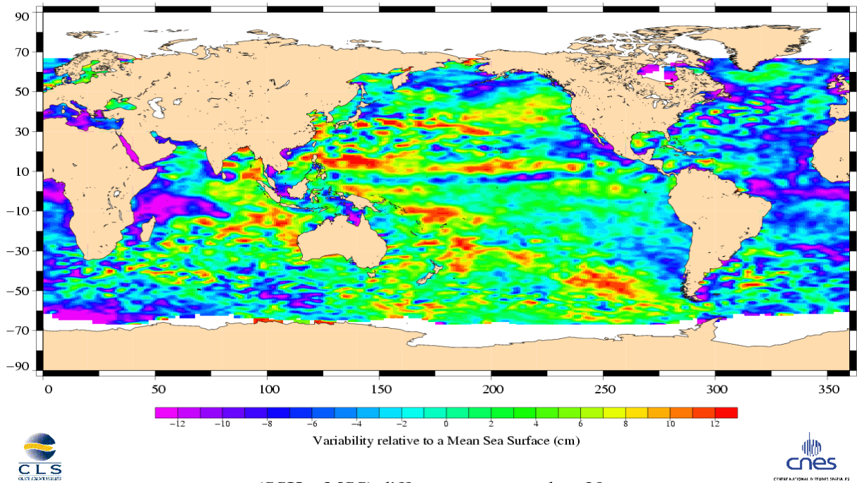
(SSH – MSS) differences greater than 30 cm Jason / Cycle 017
