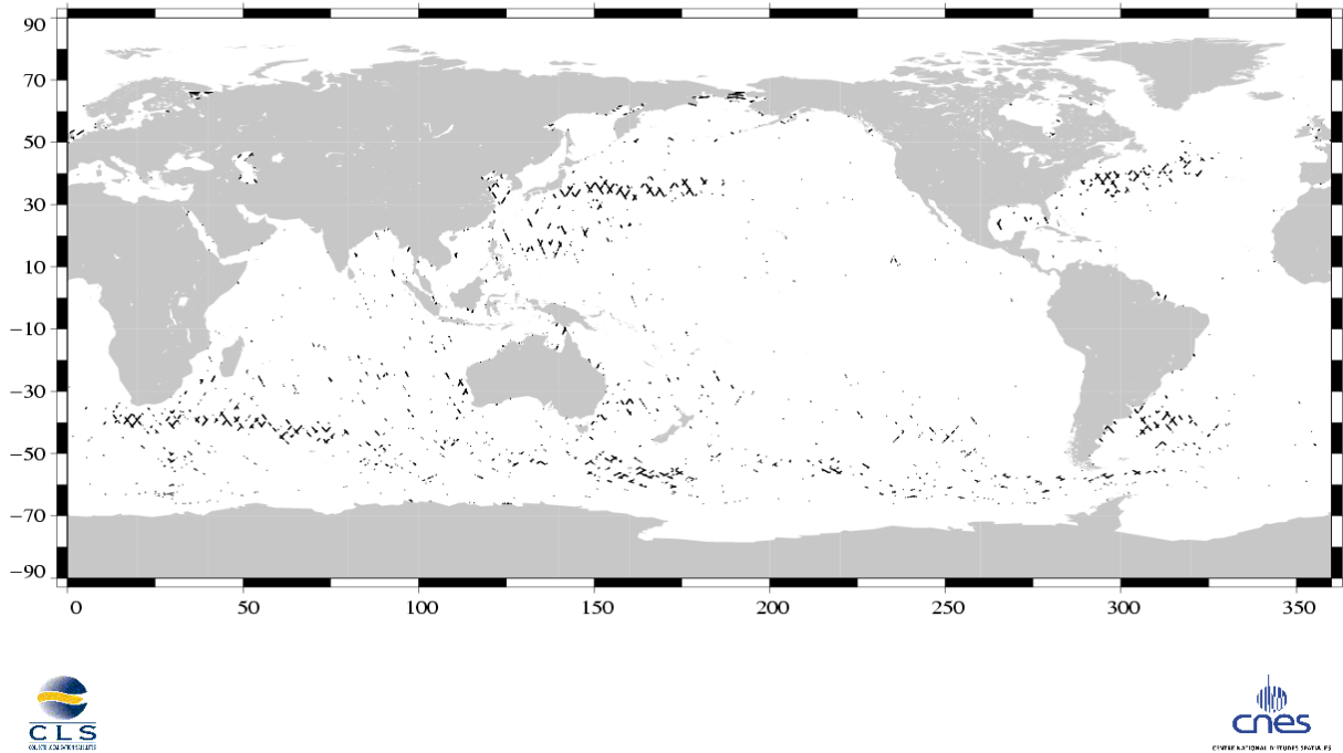
(SSH – MSS) differences greater than 30 cm Jason / Cycle 017
