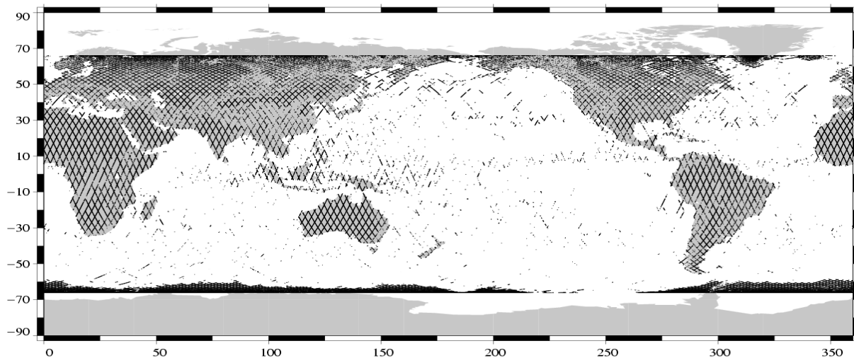
Edited measurements Jason-1 Cycle 017 (22/06/2002 / 02/07/2002)
