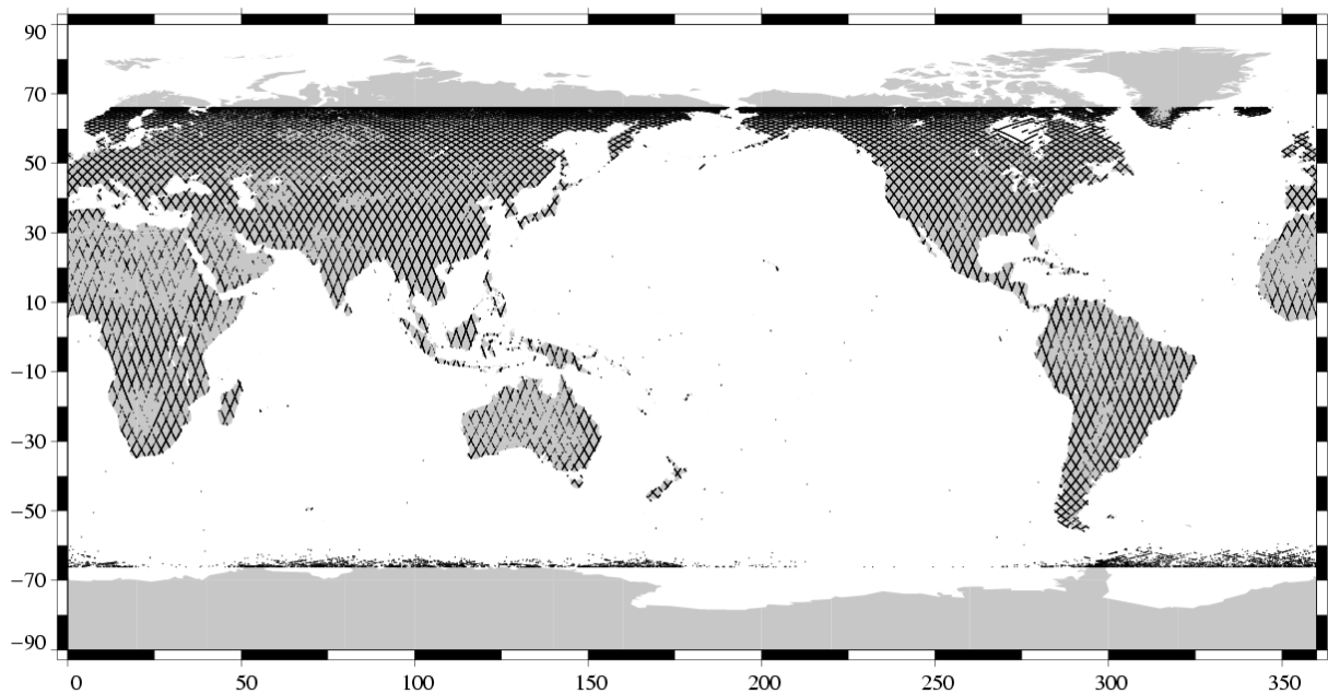
Missing measurements Jason-1 Cycle 017 (22/06/2002 / 02/07/2002)
