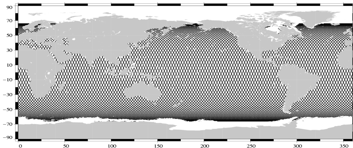
Valid data Jason-1 Cycle 017 (22/06/2002 / 02/07/2002)
