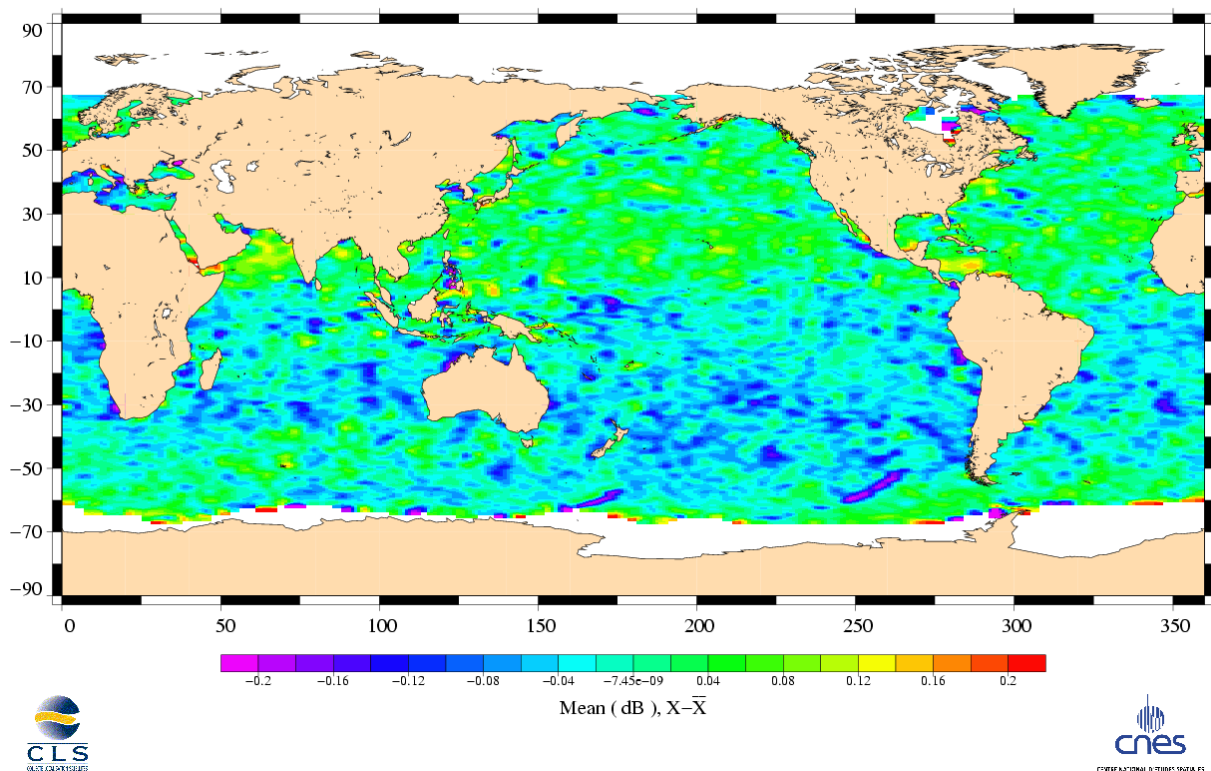
Ku SIGMA0 differences Topex (Cycle 360) – Jason (Cycle 017)
