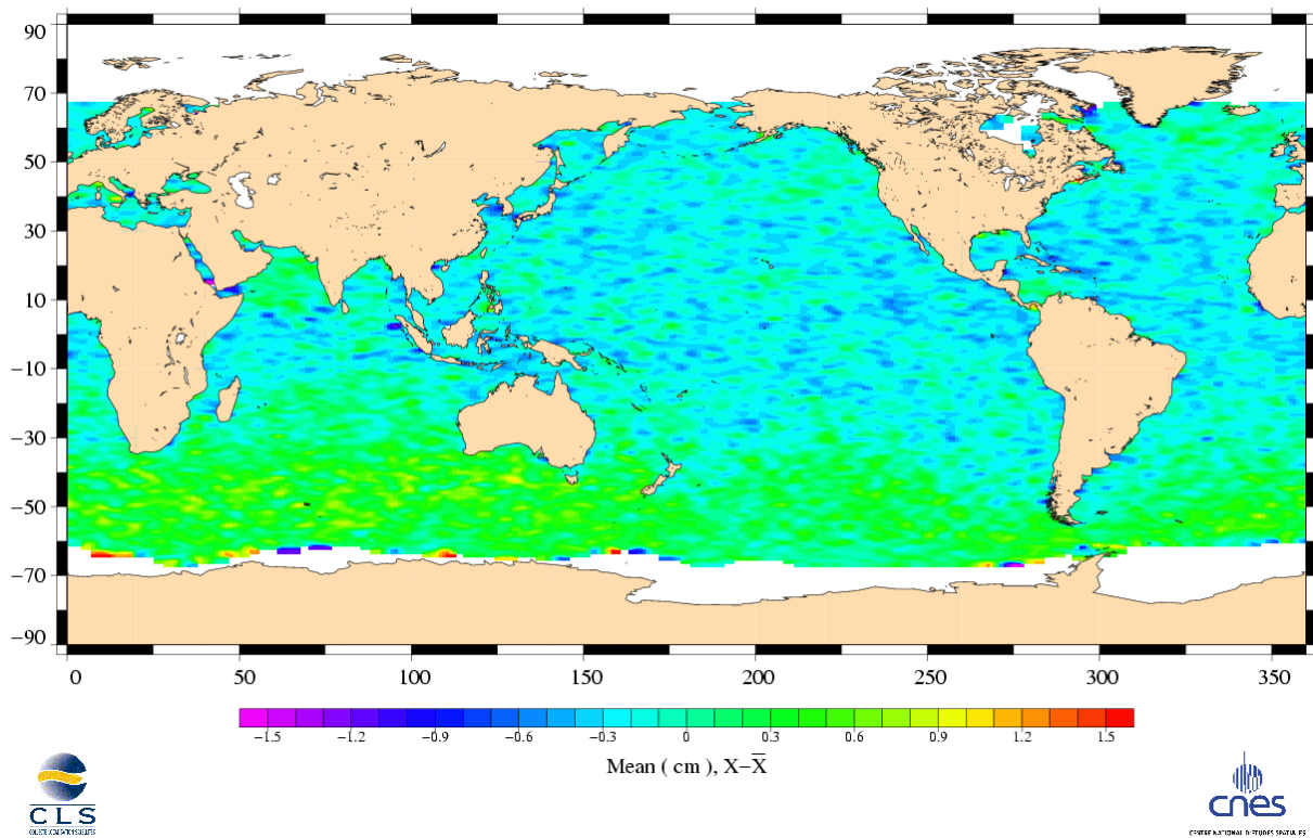
Altimeter ionospheric correction differences Topex (Cycle 360) – Jason (Cycle 017)
