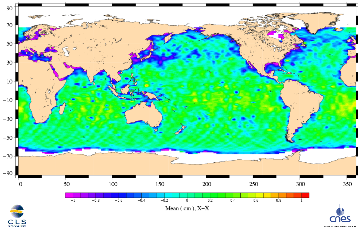
Radiometer correction differences Topex (Cycle 360) – Jason (Cycle 017)
