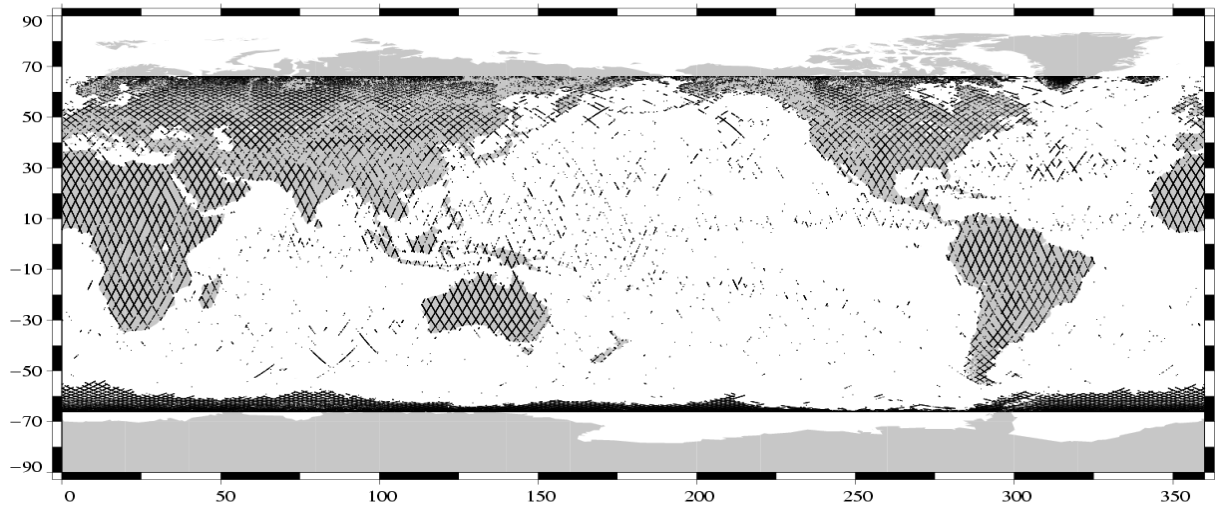
Edited measurements Jason-1 Cycle 022 (11/08/2002 / 21/08/2002)
