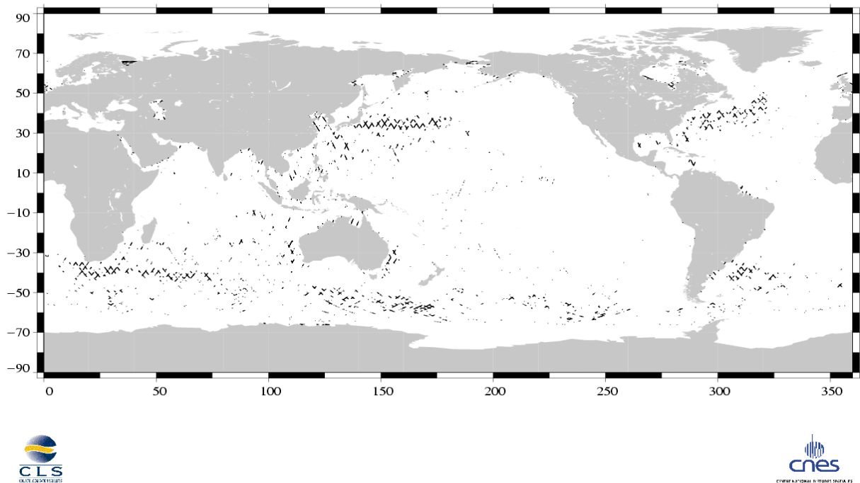
(SSH – MSS) differences greater than 30 cm Jason / Cycle 022
