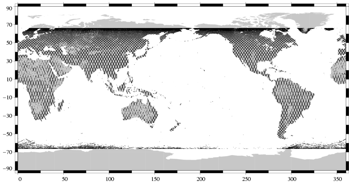
Missing measurements Jason-1 Cycle 022 (11/08/2002 / 21/08/2002)
