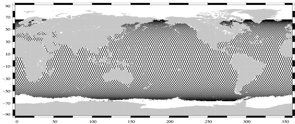
Valid data Jason-1 Cycle 022 (11/08/2002 / 21/08/2002)
