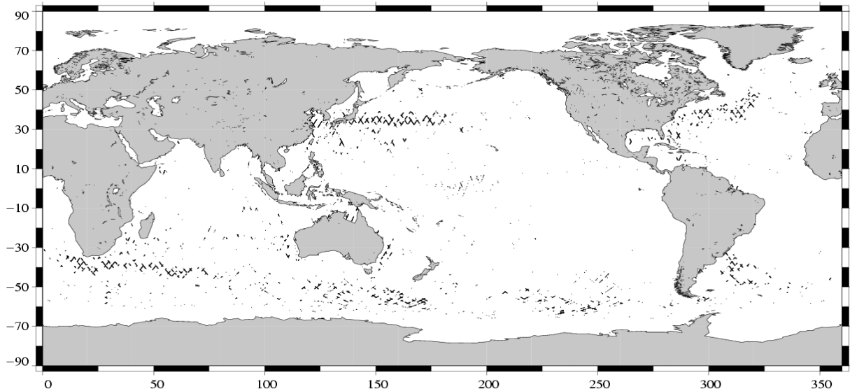
(SSH – MSS) differences greater than 30 cm Jason / Cycle 023
