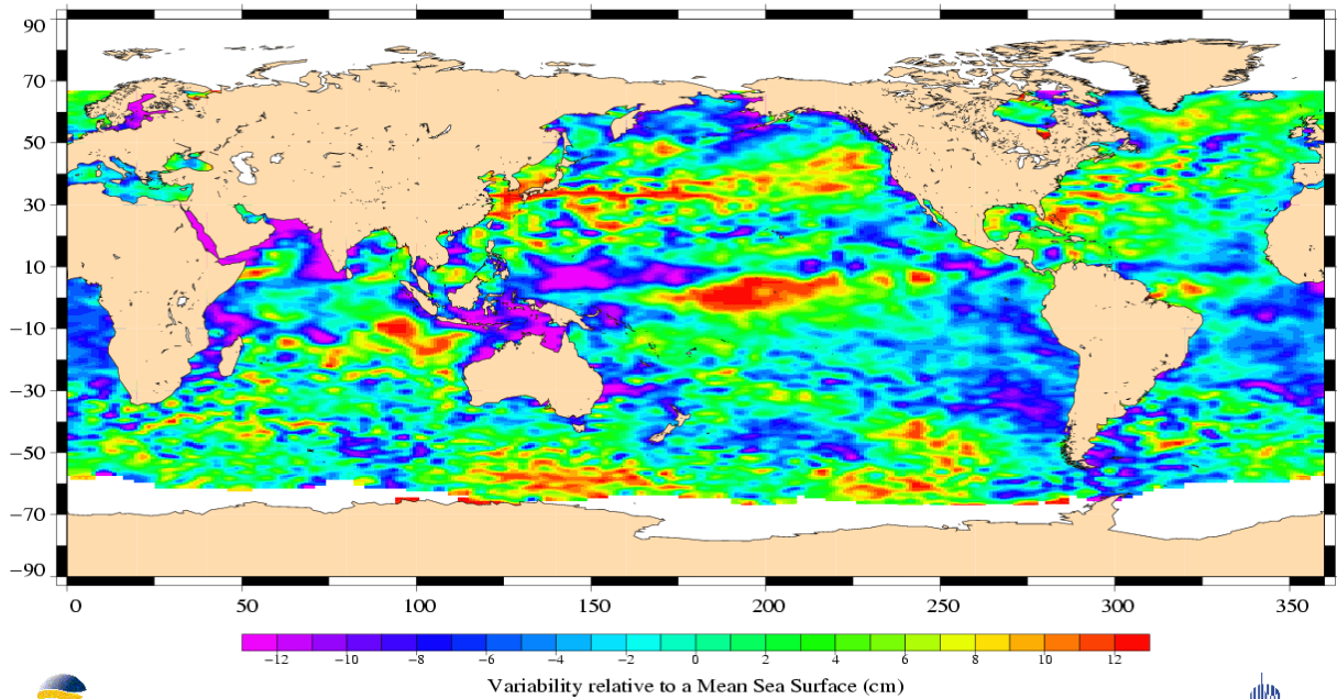
(SSH – MSS) differences greater than 30 cm Jason / Cycle 023
