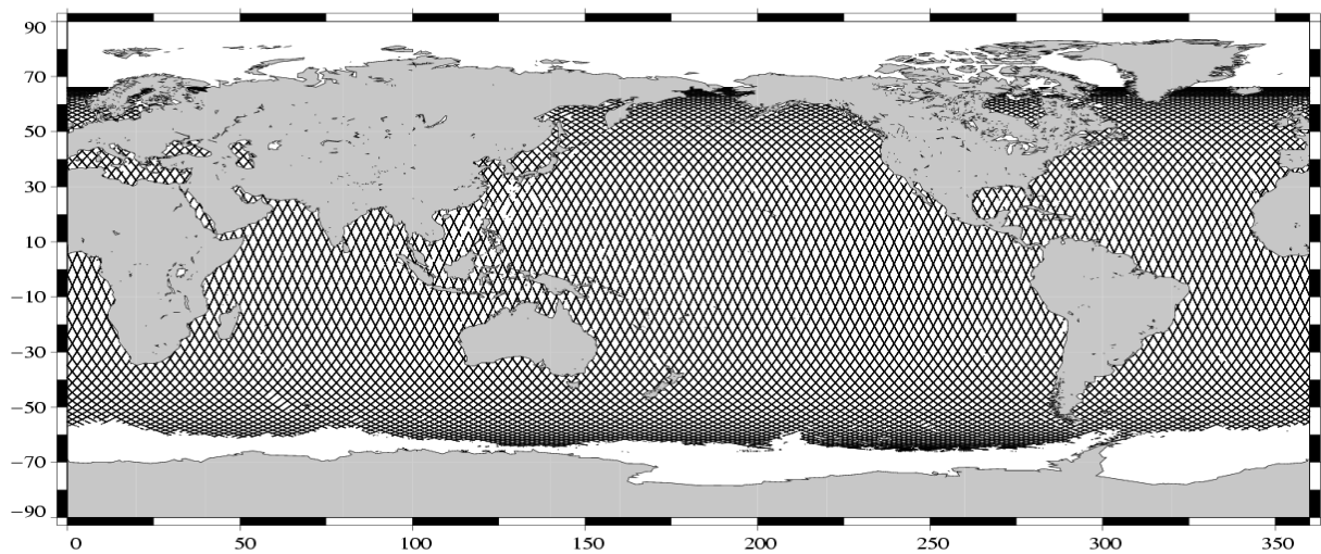
Valid data Jason-1 Cycle 023 (21/08/2002 / 31/08/2002)
