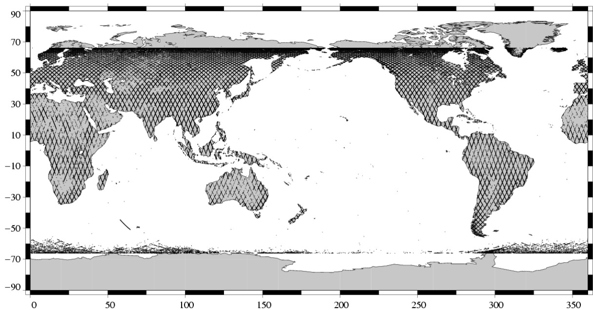
Missing measurements Jason-1 Cycle 023 (21/08/2002 / 31/08/2002)
