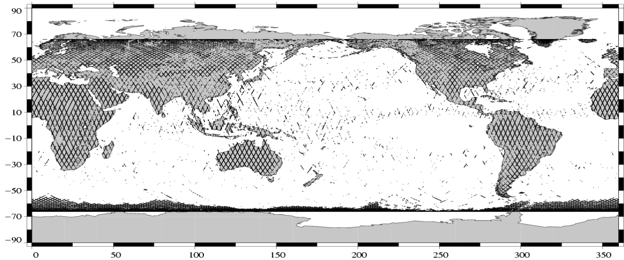
Edited measurements Jason-1 Cycle 023 (21/08/2002 / 31/08/2002)
