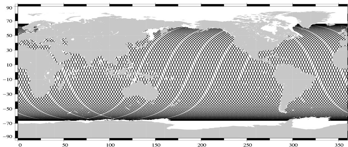
Valid data Jason-1 Cycle 046 (06/04/2003 / 16/04/2003)
