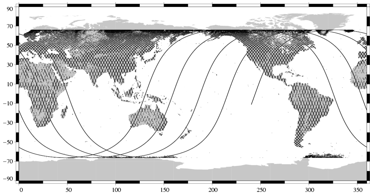
Missing measurements Jason-1 Cycle 046 (06/04/2003 / 16/04/2003)
