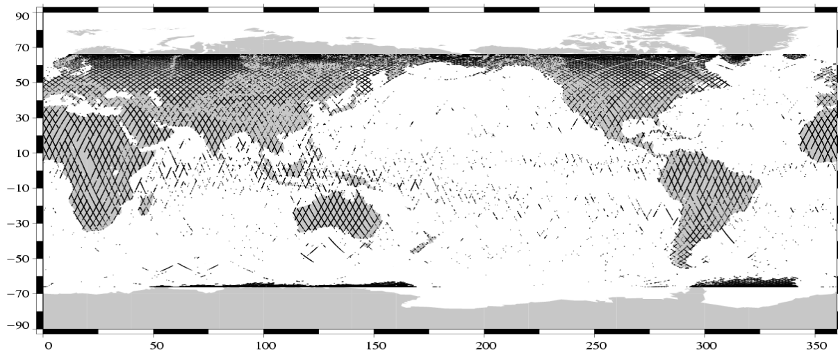
Edited measurements Jason-1 Cycle 046 (06/04/2003 / 16/04/2003)
