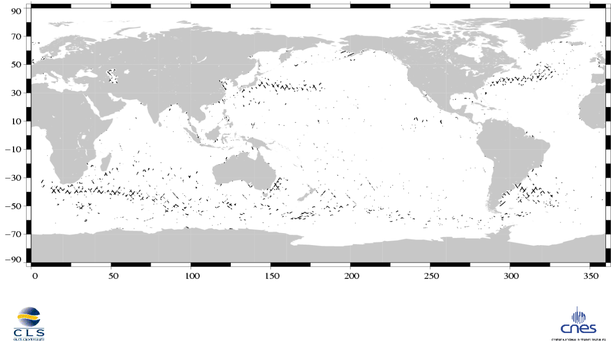
(SSH – MSS) differences greater than 30 cm Jason / Cycle 046
