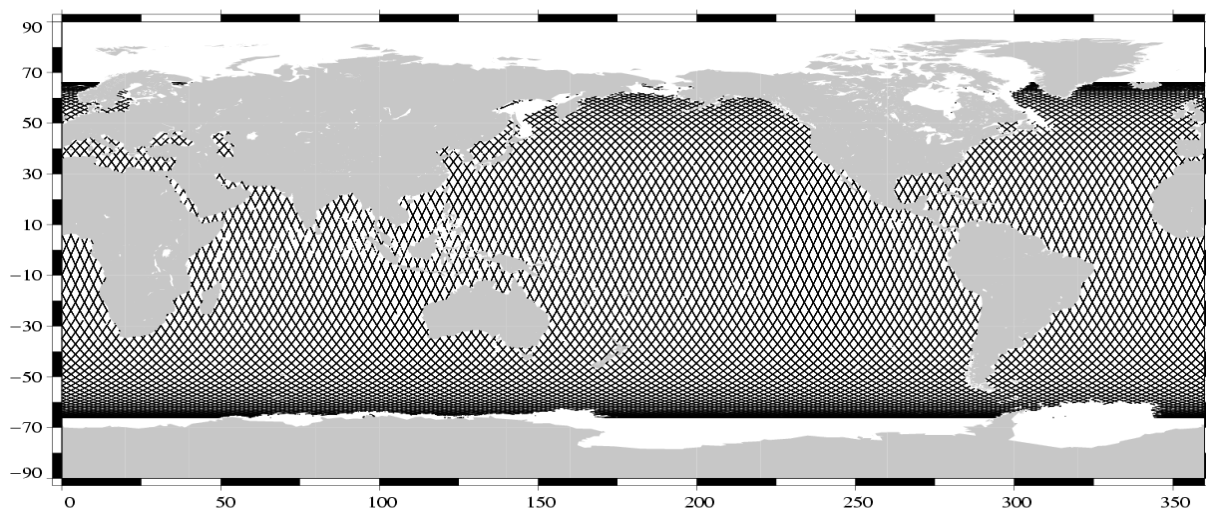
Valid data Jason-1 Cycle 047 (16/04/2003 / 26/04/2003)
