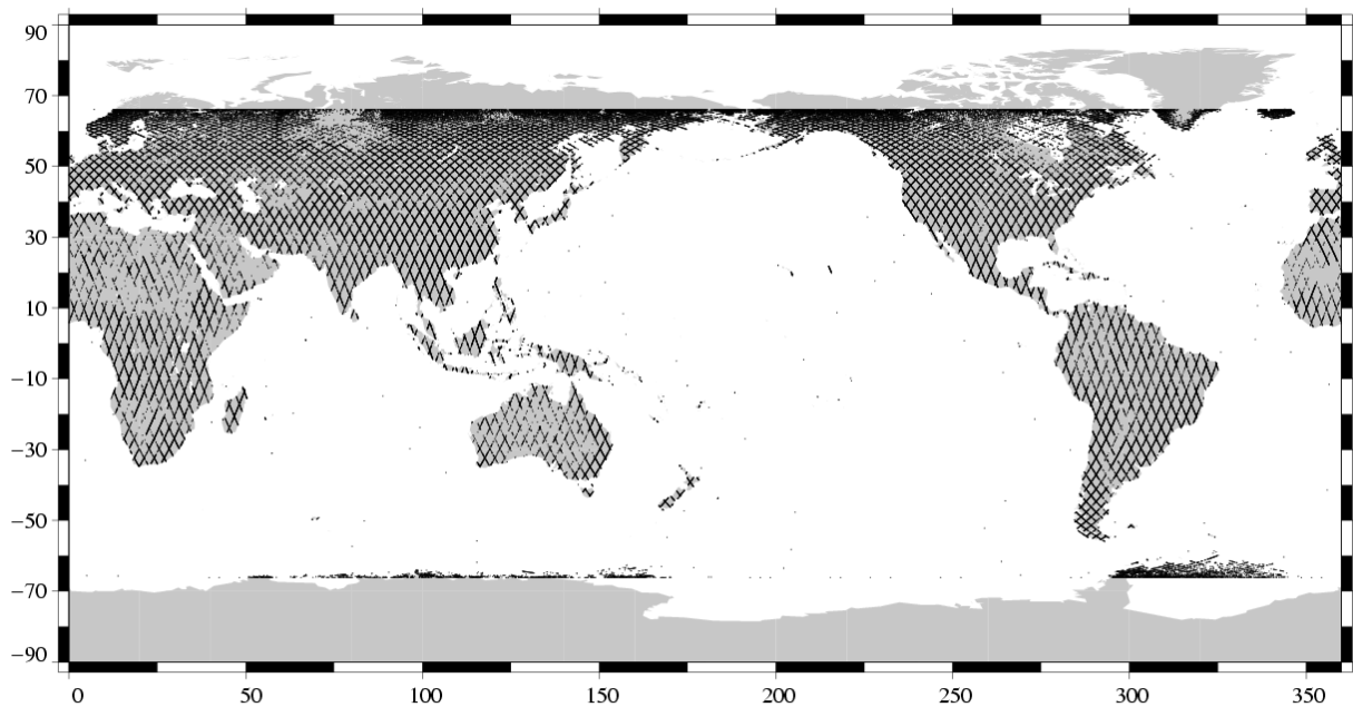
Missing measurements Jason-1 Cycle 047 (16/04/2003 / 26/04/2003)
