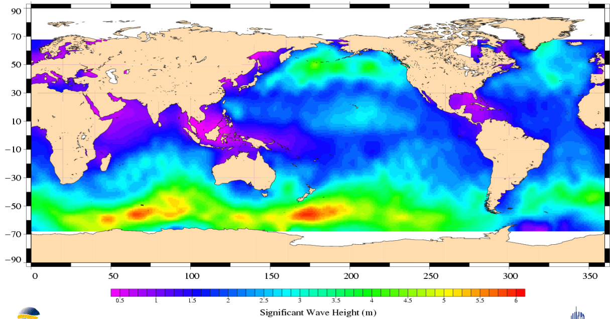
Jason-1 Cycle 047 16/04/2003 – 26/04/2003
