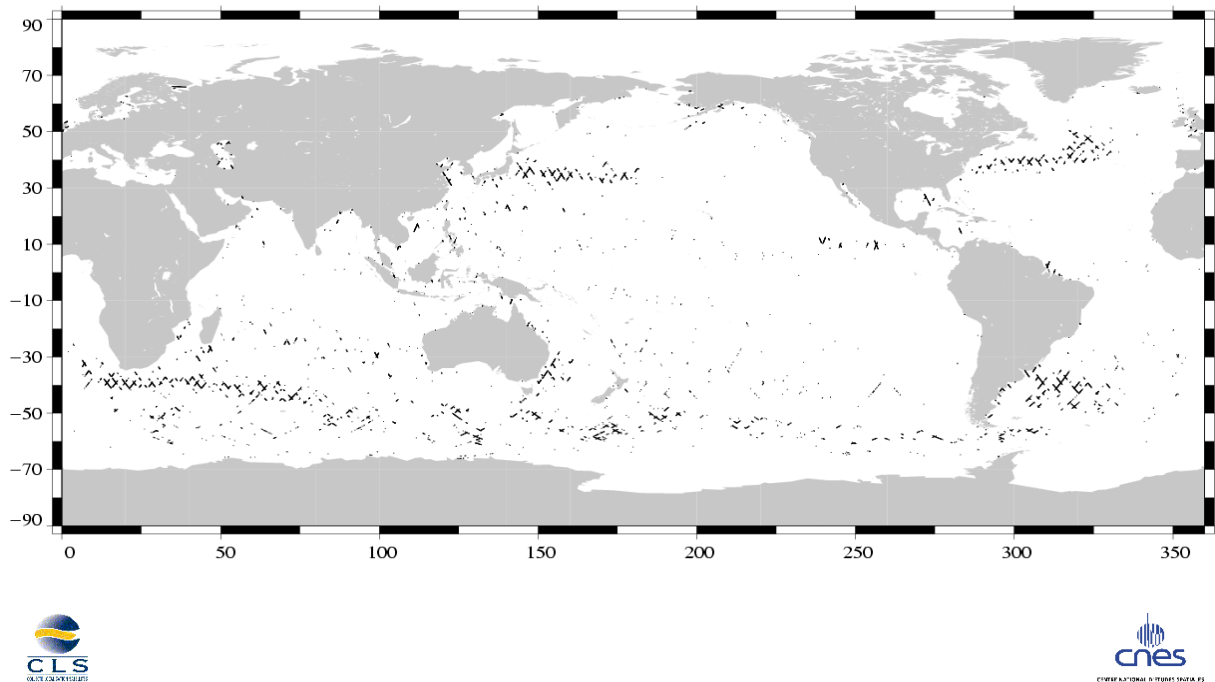
(SSH – MSS) differences greater than 30 cm Jason / Cycle 047
