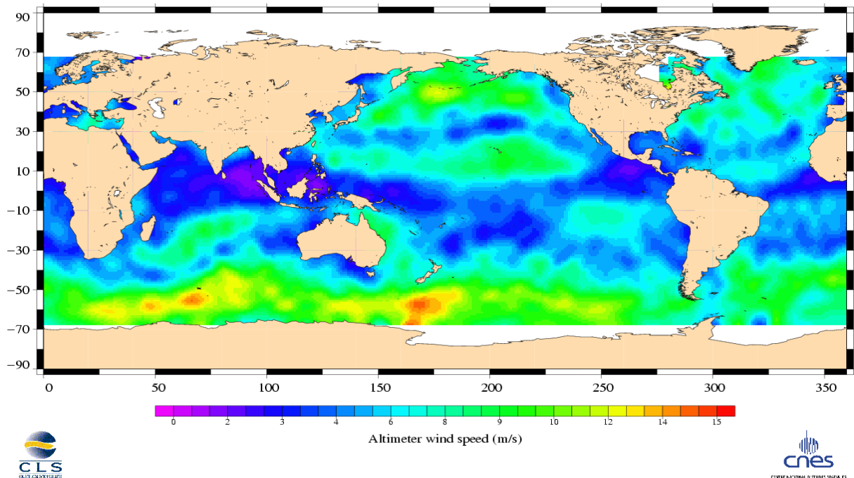
Jason-1 Cycle 047 16/04/2003 – 26/04/2003
