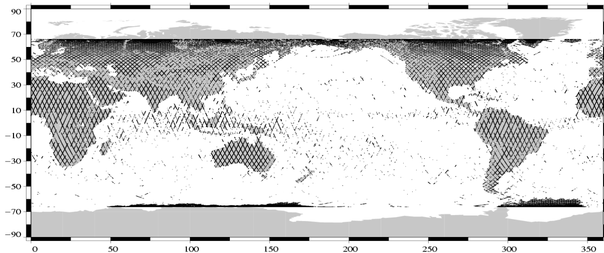
Edited measurements Jason-1 Cycle 047 (16/04/2003 / 26/04/2003)
