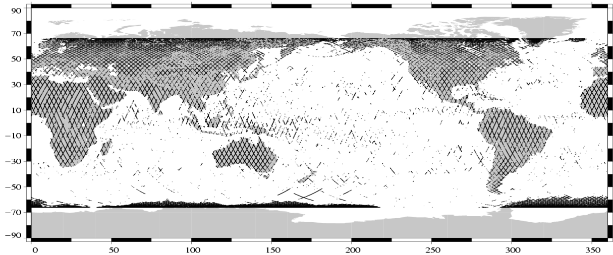
Edited measurements Jason-1 Cycle 051 (25/05/2003 / 04/06/2003)
