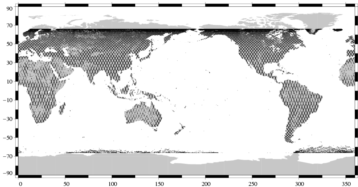
Missing measurements Jason-1 Cycle 051 (25/05/2003 / 04/06/2003)
