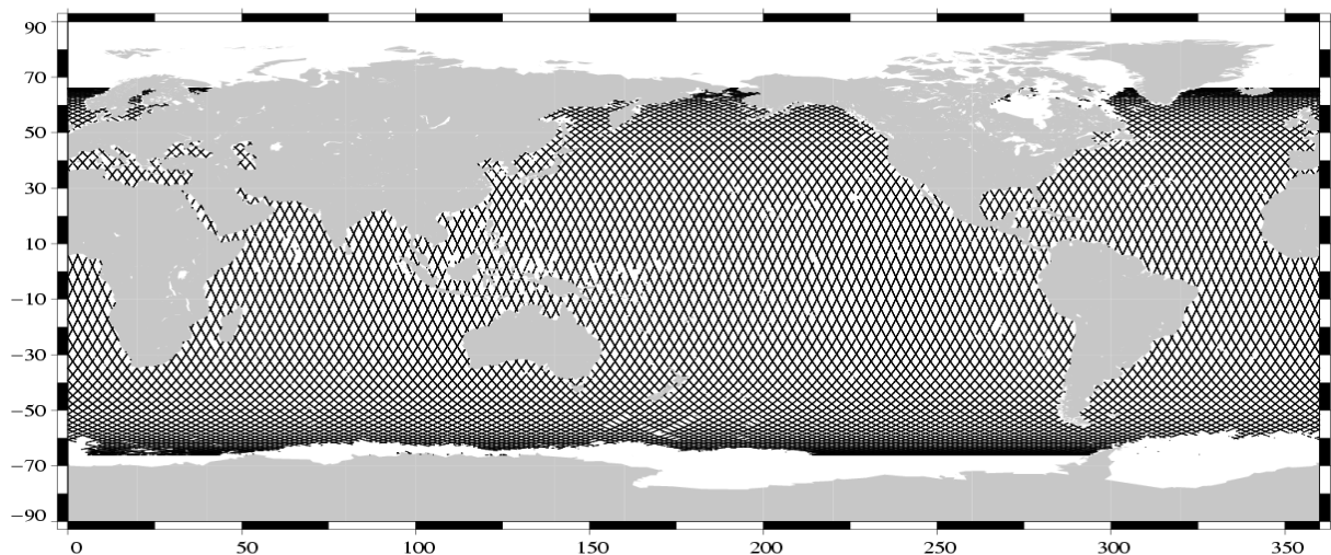
Valid data Jason-1 Cycle 051 (25/05/2003 / 04/06/2003)
