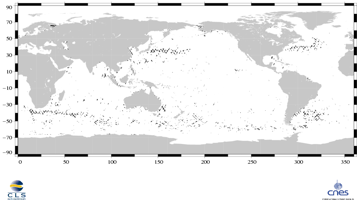
(SSH – MSS) differences greater than 30 cm Jason / Cycle 051
