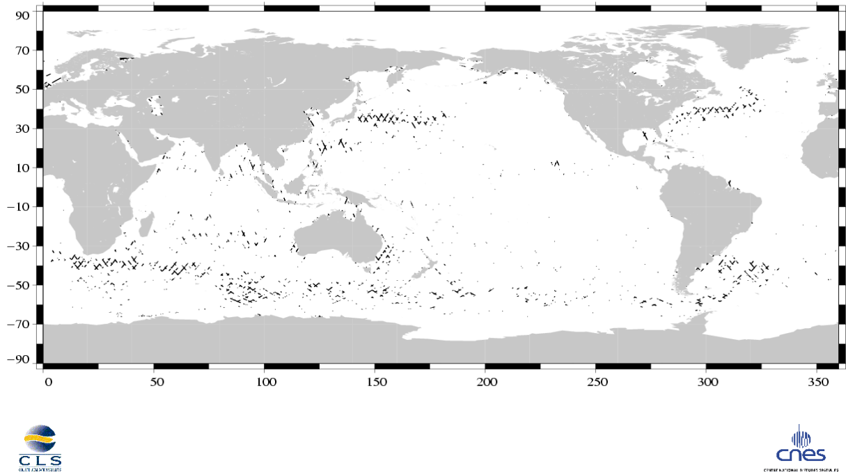
(SSH – MSS) differences greater than 30 cm Jason / Cycle 053
