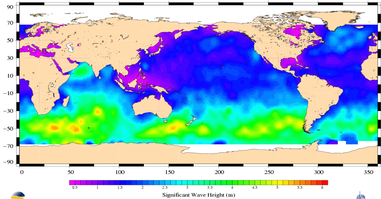
Jason-1 Cycle 053 14/06/2003 – 24/06/2003
