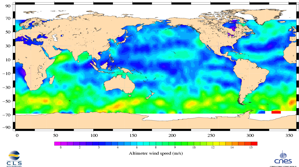
Jason-1 Cycle 053 14/06/2003 – 24/06/2003
