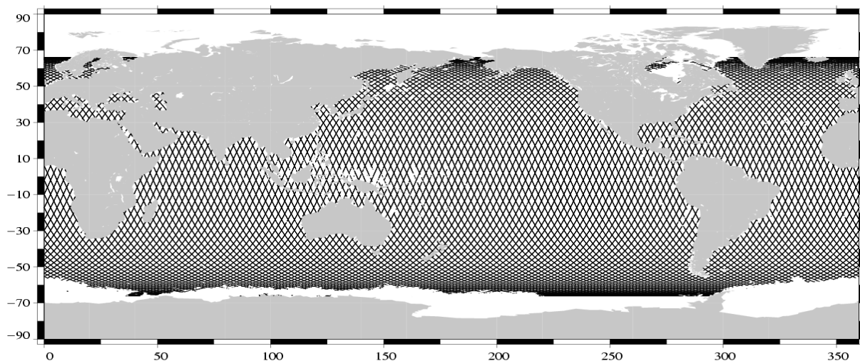
Valid data Jason-1 Cycle 054 (24/06/2003 / 04/07/2003)
