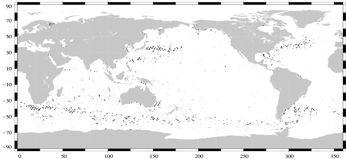
(SSH – MSS) differences greater than 30 cm Jason / Cycle 054
