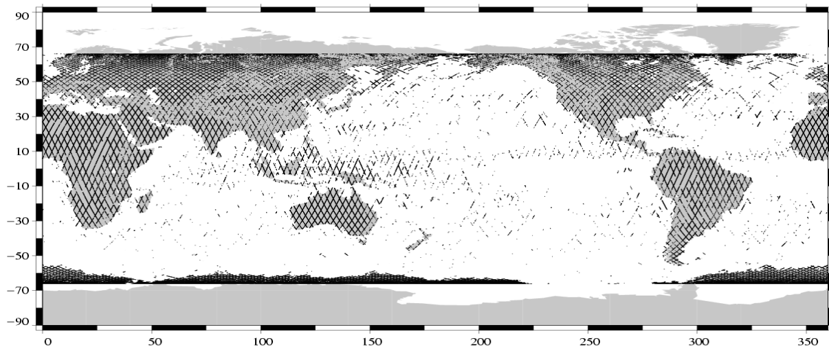
Edited measurements Jason-1 Cycle 054 (24/06/2003 / 04/07/2003)
