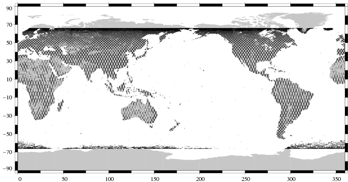
Missing measurements Jason-1 Cycle 054 (24/06/2003 / 04/07/2003)
