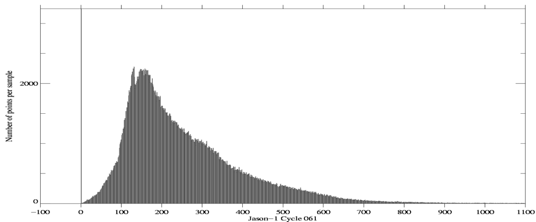
Ku-band Significant Wave Height ( unit : cm)
