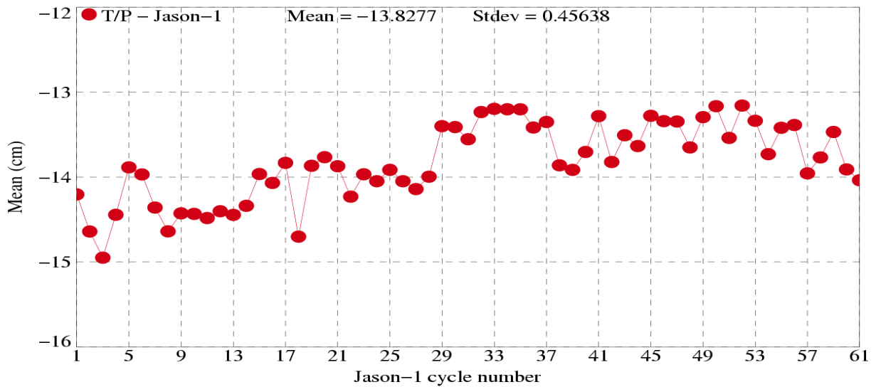
Crossover mean
