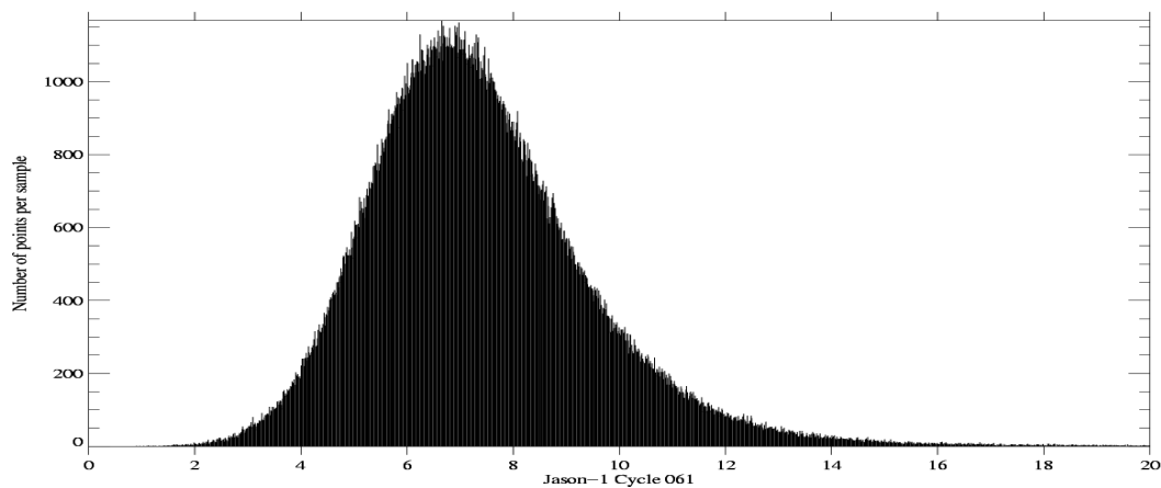
RMS of Ku-band range ( unit : cm)
