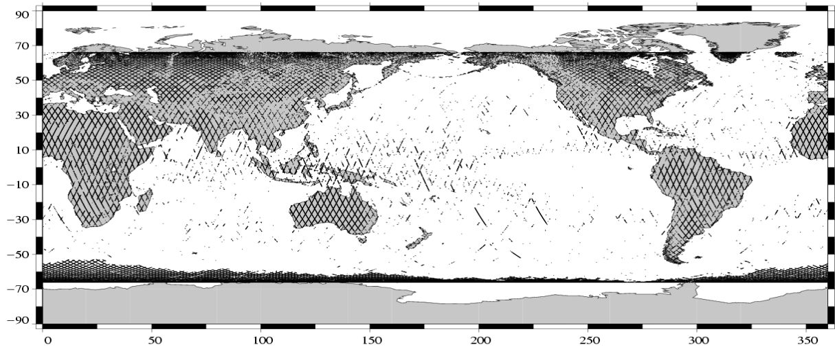
Edited measurements Jason-1 Cycle 066 (21/10/2003 / 31/10/2003)
