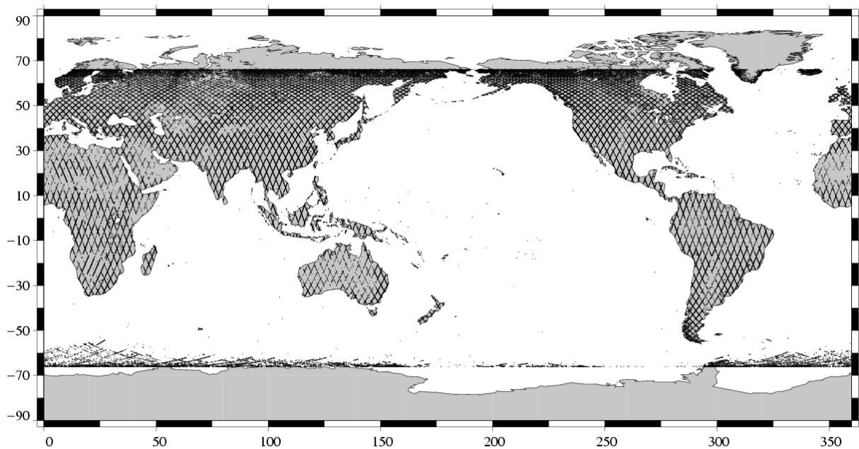
Missing measurements Jason-1 Cycle 066 (21/10/2003 / 31/10/2003)
