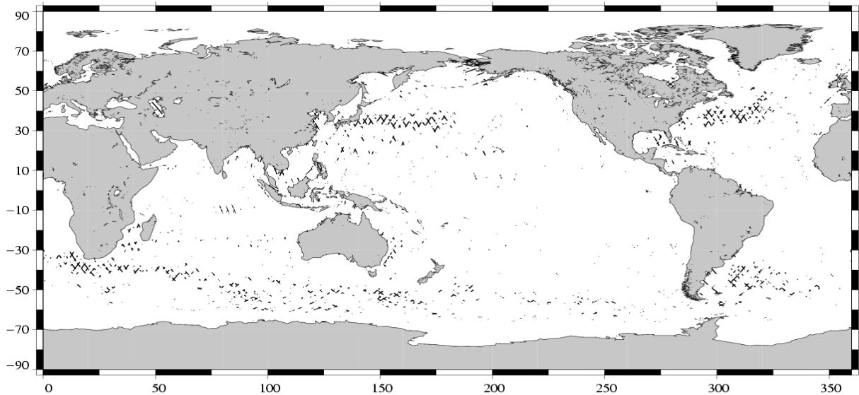
(SSH – MSS) differences greater than 30 cm Jason / Cycle 066
