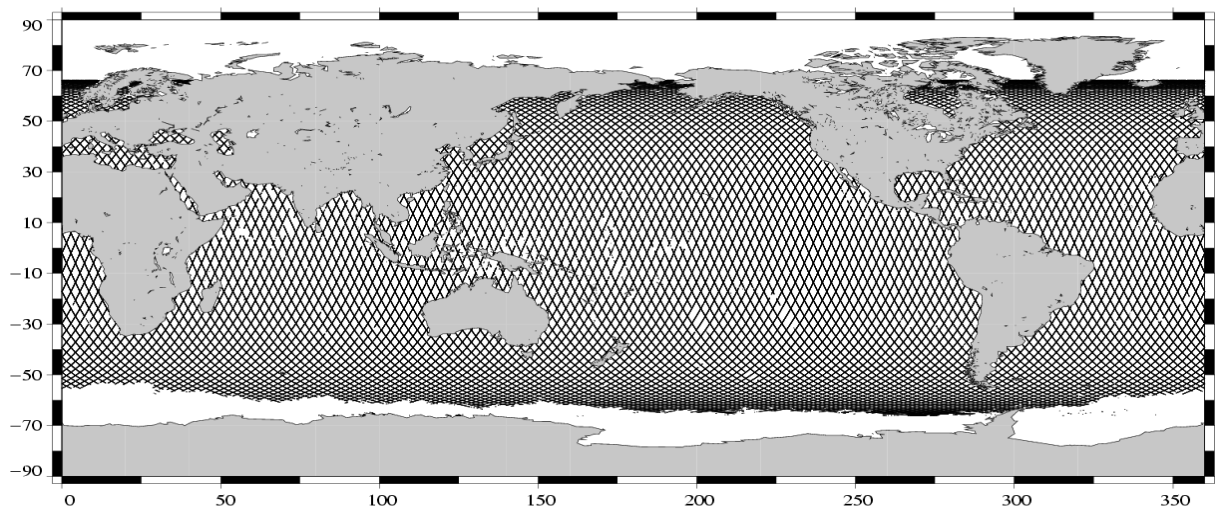
Valid data Jason-1 Cycle 066 (21/10/2003 / 31/10/2003)
