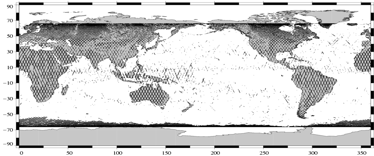
Edited measurements Jason-1 Cycle 067 (31/10/2003 / 10/11/2003)
