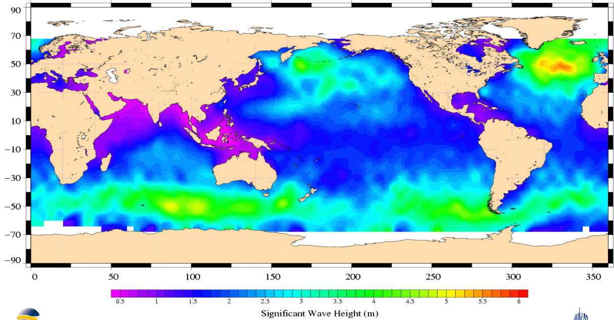
Jason-1 Cycle 067 31/10/2003 – 10/11/2003
