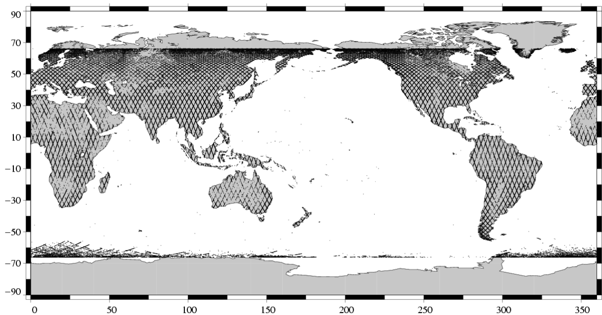
Missing measurements Jason-1 Cycle 067 (31/10/2003 / 10/11/2003)
