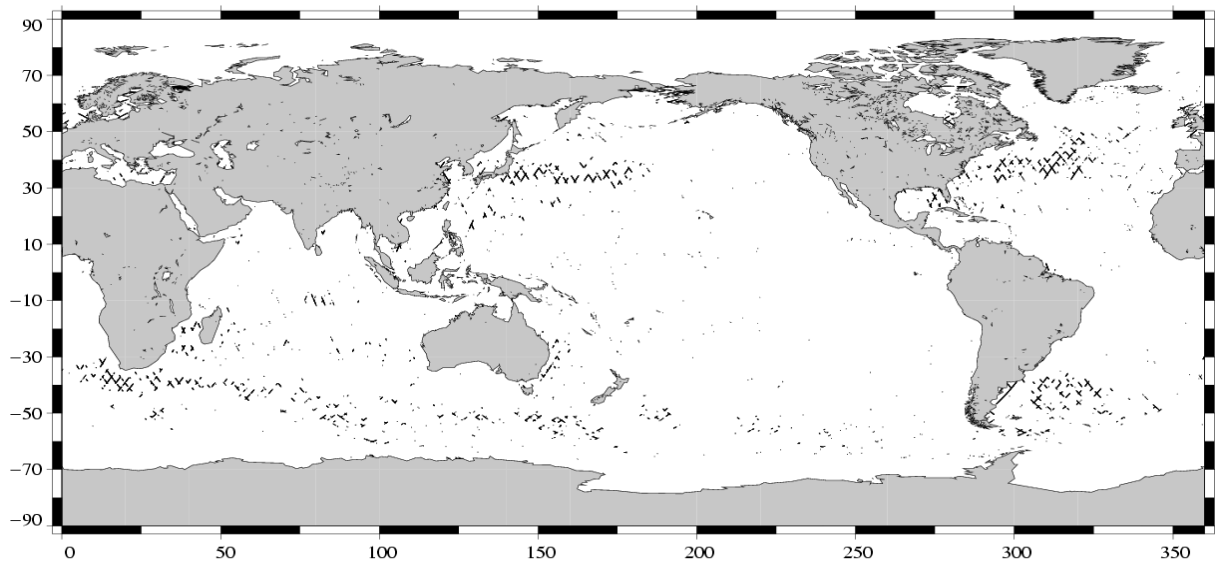
(SSH – MSS) differences greater than 30 cm Jason / Cycle 067
