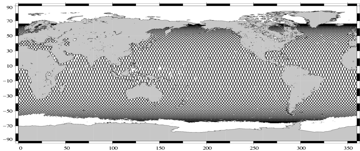
Valid data Jason-1 Cycle 067 (31/10/2003 / 10/11/2003)
