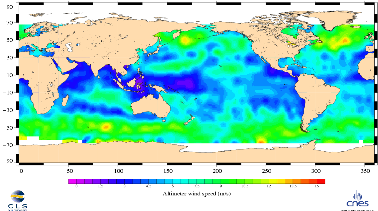
Jason-1 Cycle 067 31/10/2003 – 10/11/2003
