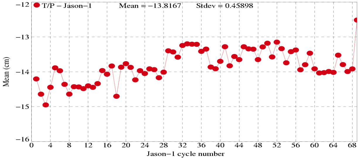
Crossover mean
