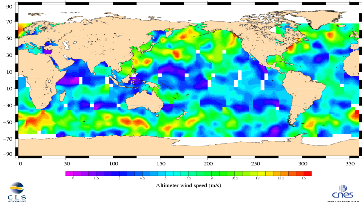
Jason-1 Cycle 069 28/11/2003 – 30/11/2003
