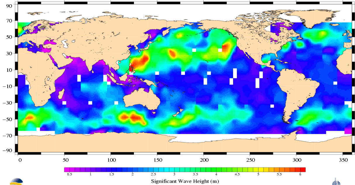
Jason-1 Cycle 069 28/11/2003 – 30/11/2003
