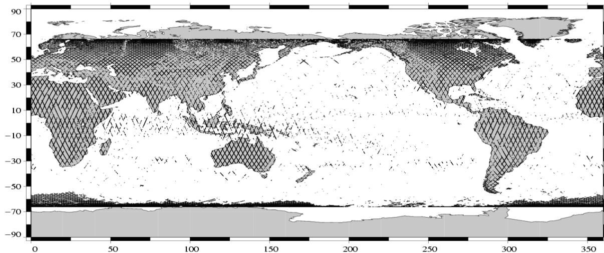
Edited measurements Jason-1 Cycle 070 (30/11/2003 / 10/12/2003)
