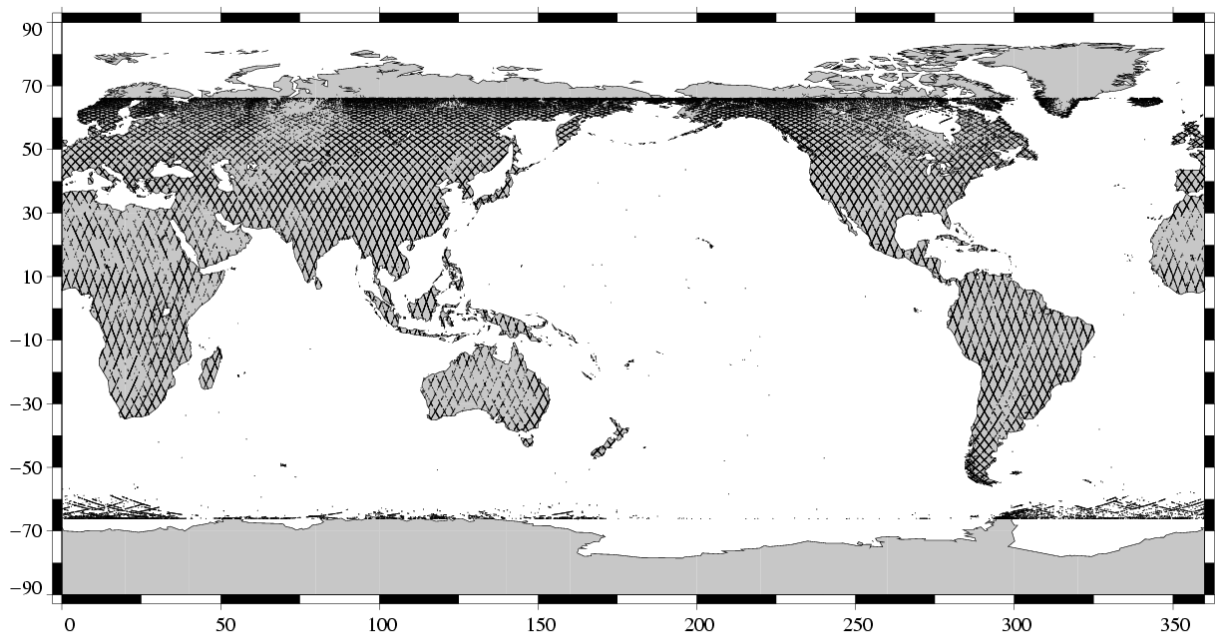
Missing measurements Jason-1 Cycle 070 (30/11/2003 / 10/12/2003)
