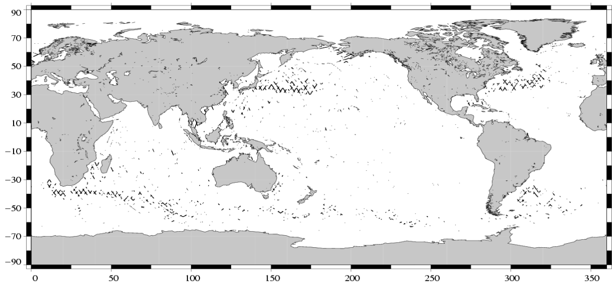
(SSH – MSS) differences greater than 30 cm Jason / Cycle 070
