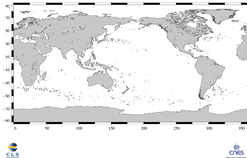
(SSH – MSS) differences greater than 30 cm Jason / Cycle 078
