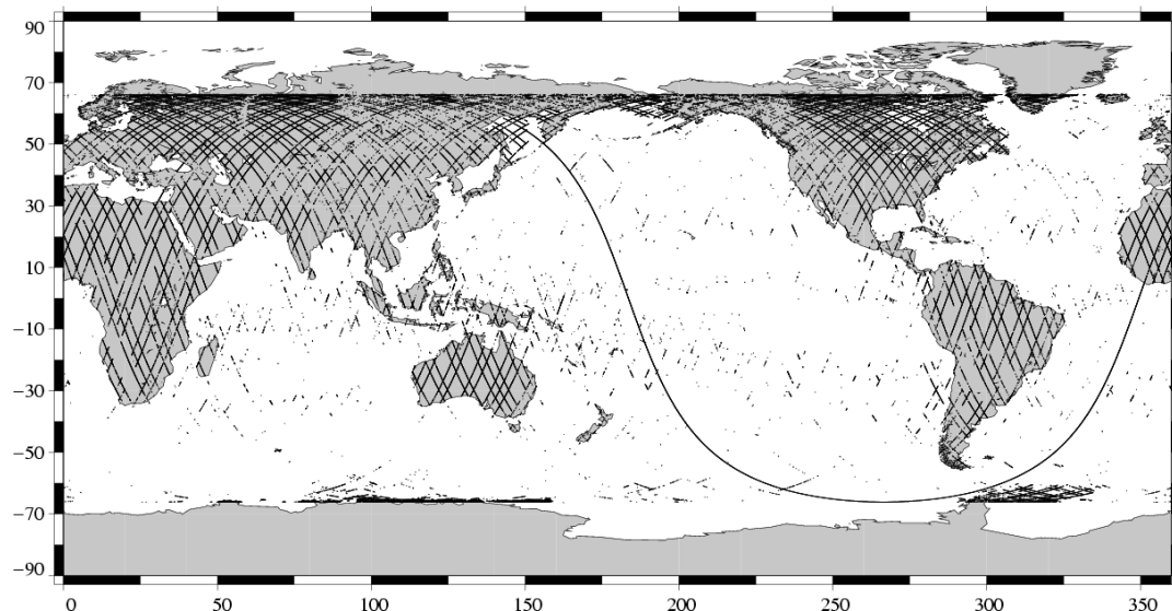
Edited measurements Jason-1 Cycle 078 (20/02/2004 / 27/02/2004)
