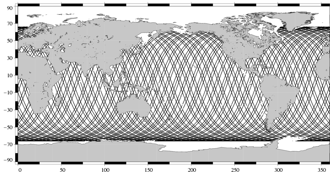
Valid data Jason-1 Cycle 078 (20/02/2004 / 27/02/2004)
