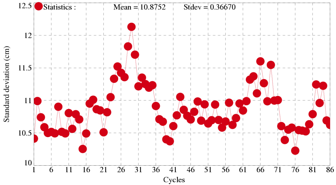
Standard deviation of Sea Level Anomalies
