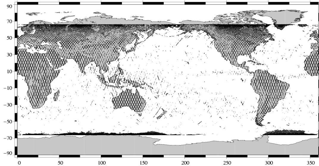
Edited measurements Jason-1 Cycle 086 (07/05/2004 / 16/05/2004)
