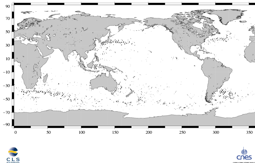
(SSH – MSS) differences greater than 30 cm Jason / Cycle 086
