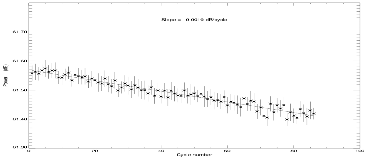
POSEIDON2 – Cycle 086
