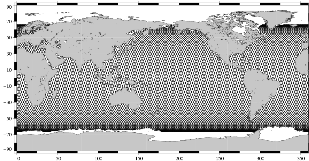
Valid data Jason-1 Cycle 086 (07/05/2004 / 16/05/2004)
