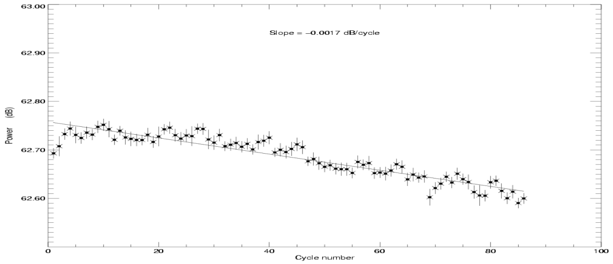
POSEIDON2 – Cycle 086
