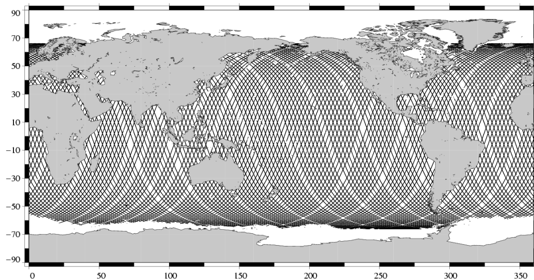
Valid data Jason-1 Cycle 091 (25/06/2004 / 05/07/2004)
