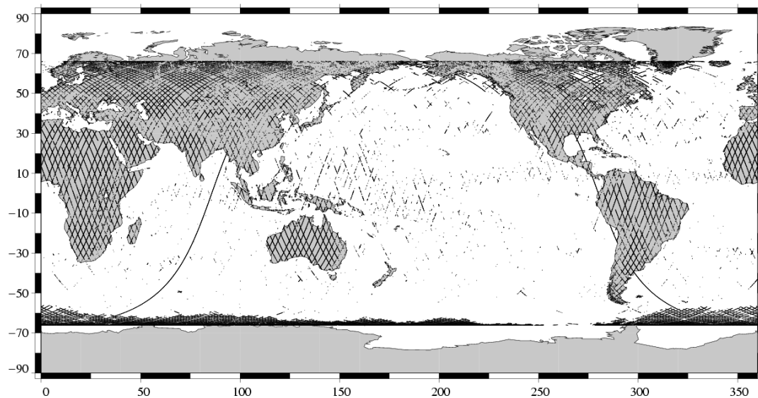
Edited measurements Jason-1 Cycle 091 (25/06/2004 / 05/07/2004)
