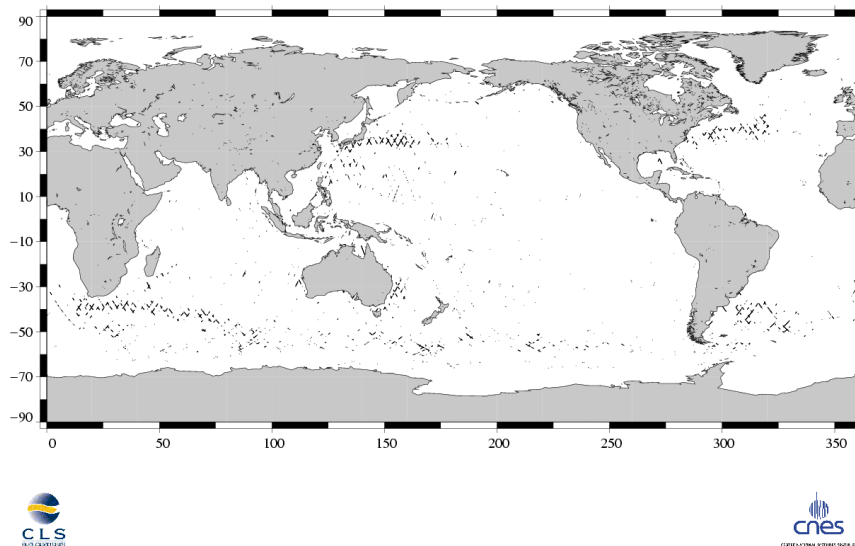
(SSH – MSS) differences greater than 30 cm Jason / Cycle 091
