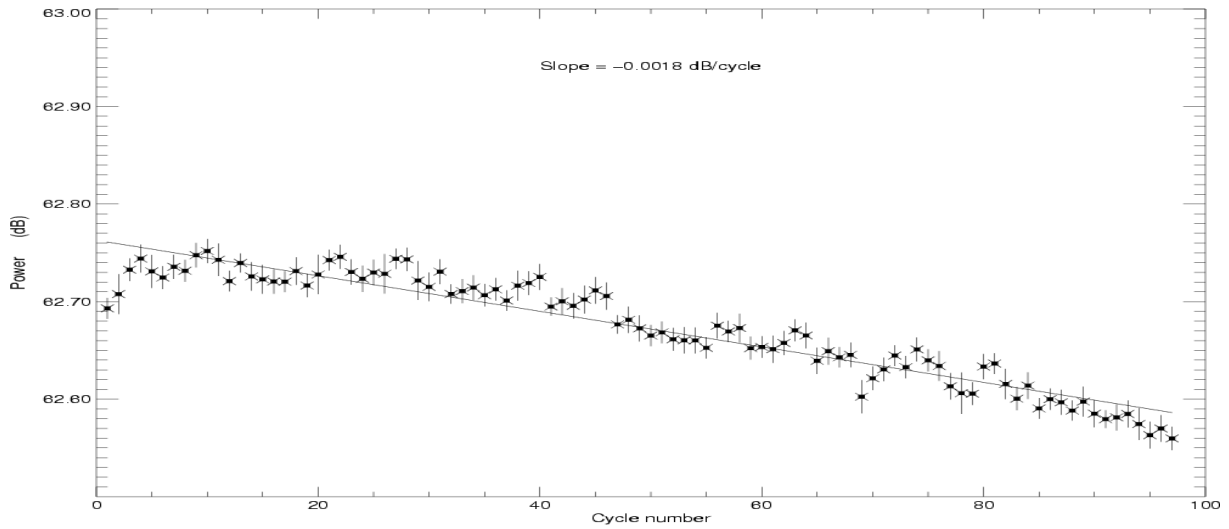
POSEIDON2 – Cycle 097
