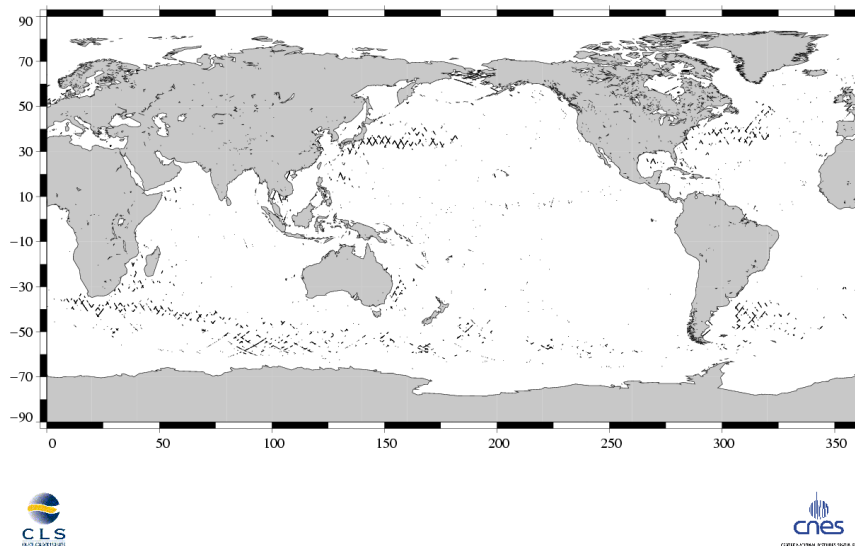
(SSH - MSS) differences greater than 30 cm Jason / Cycle 103
