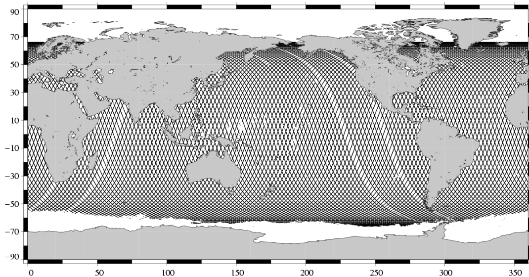
Valid data Jason-1 Cycle 103 (22/10/2004 / 01/11/2004)
