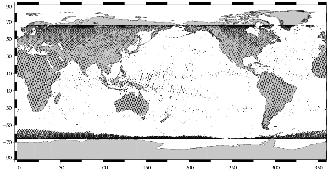
Edited measurements Jason-1 Cycle 103 (22/10/2004 / 01/11/2004)
