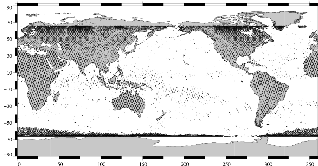
Edited measurements Jason-1 Cycle 106 (21/11/2004 / 01/12/2004)
