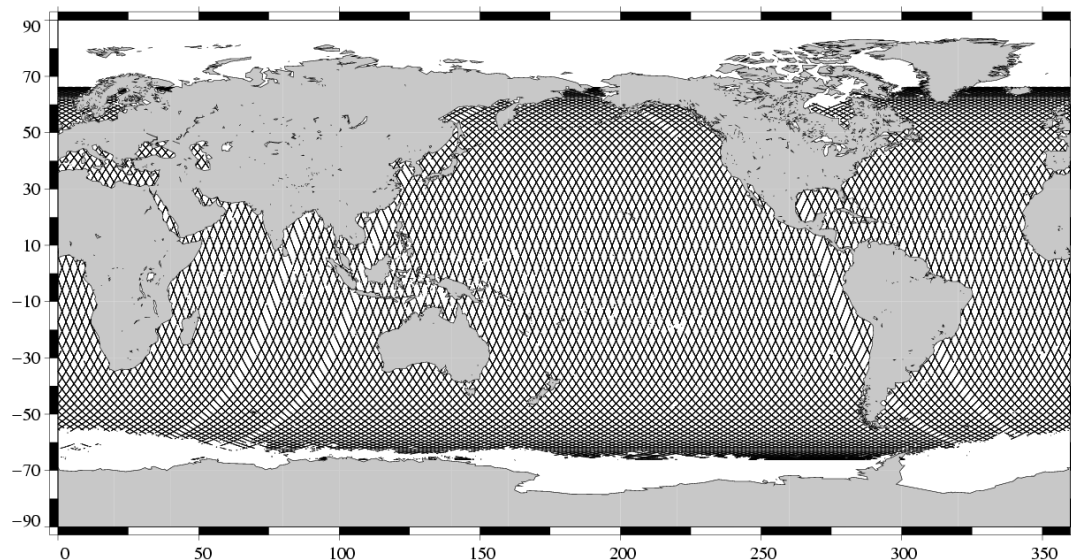
Valid data Jason-1 Cycle 106 (21/11/2004 / 01/12/2004)
