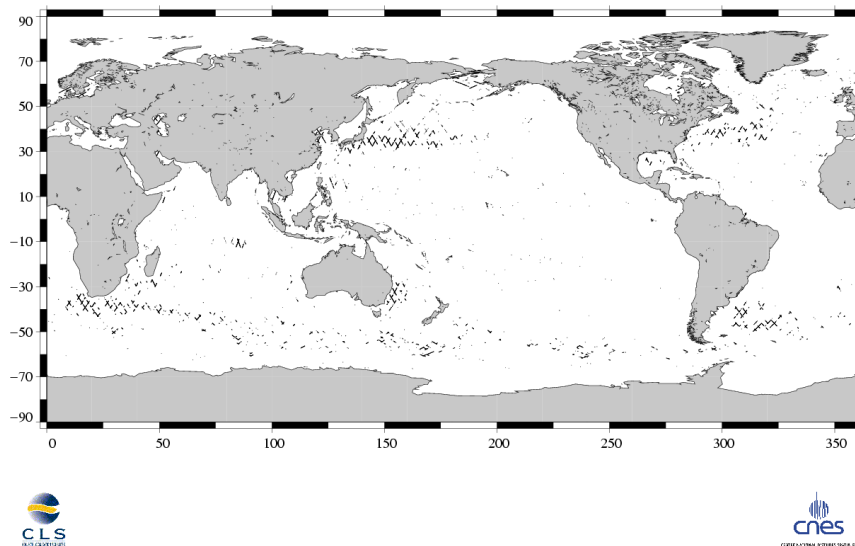
(SSH - MSS) differences greater than 30 cm Jason / Cycle 106
