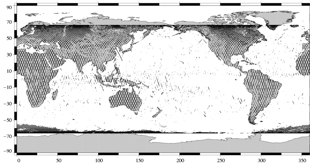
Edited measurements Jason-1 Cycle 107 (01/12/2004 / 11/12/2004)
