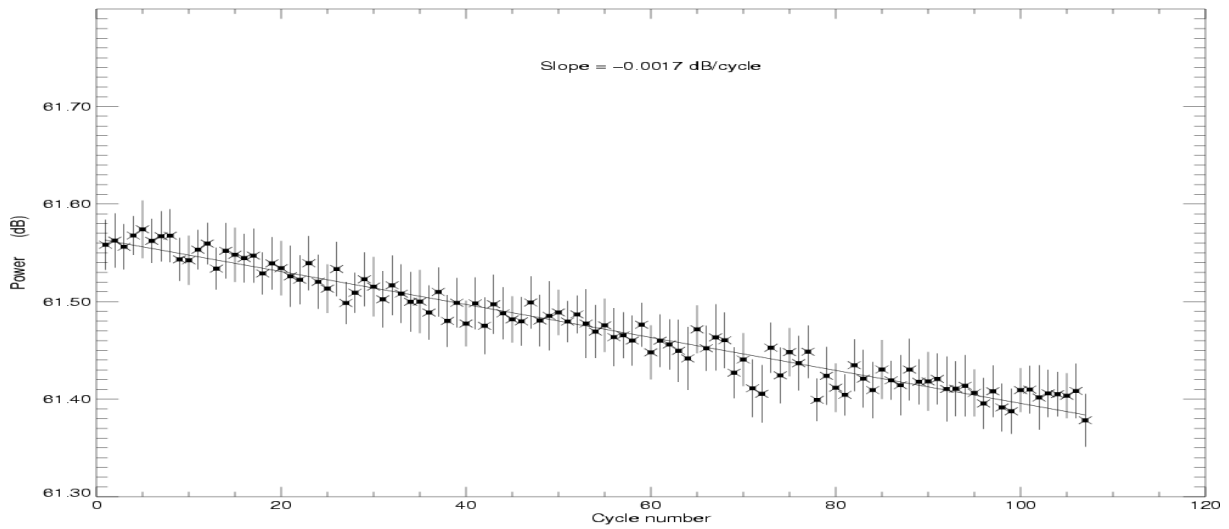
POSEIDON2 – Cycle 107
