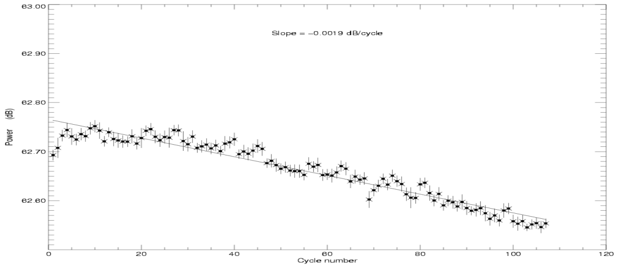
POSEIDON2 – Cycle 107
