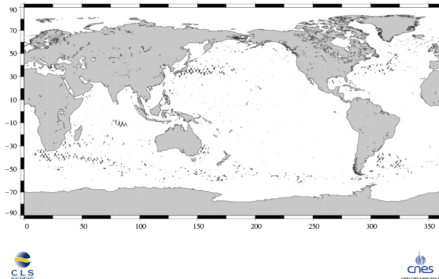
(SSH – MSS) differences greater than 30 cm Jason / Cycle 107
