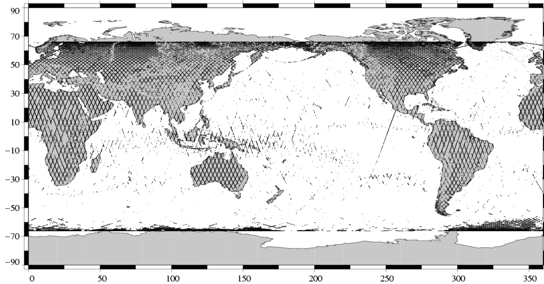
Edited measurements Jason-1 Cycle 109 (21/12/2004 / 31/12/2004)
