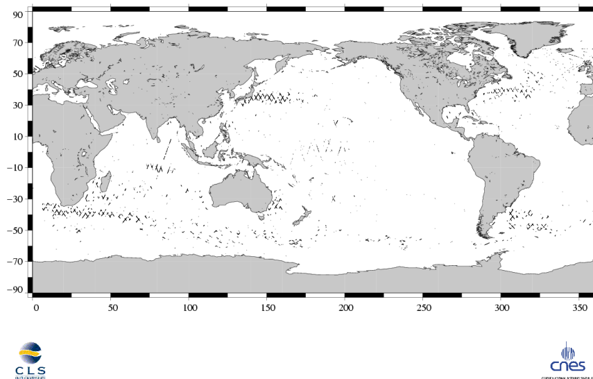
(SSH – MSS) differences greater than 30 cm Jason / Cycle 109
