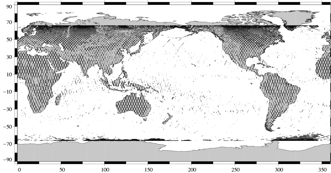
Edited measurements Jason-1 Cycle 110 (31/12/2004 / 09/01/2005)
