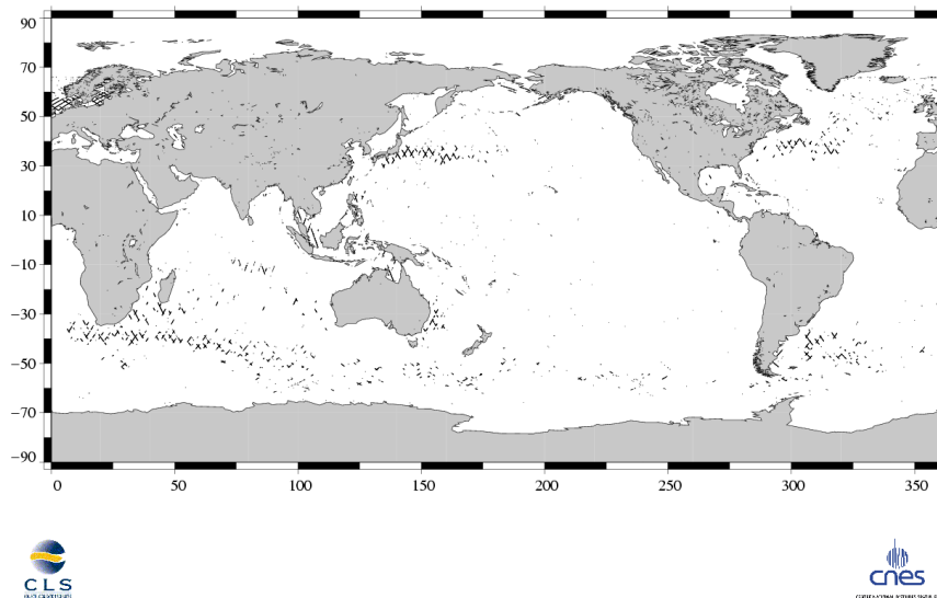
(SSH - MSS) differences greater than 30 cm Jason / Cycle 110
