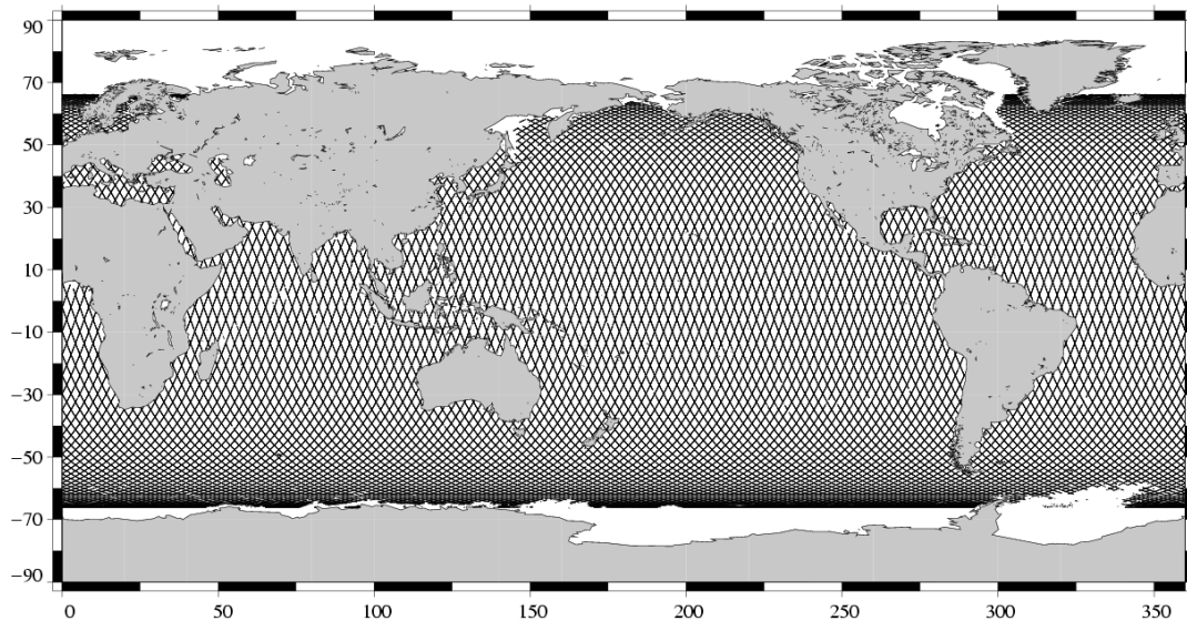
Valid data Jason-1 Cycle 110 (31/12/2004 / 09/01/2005)
