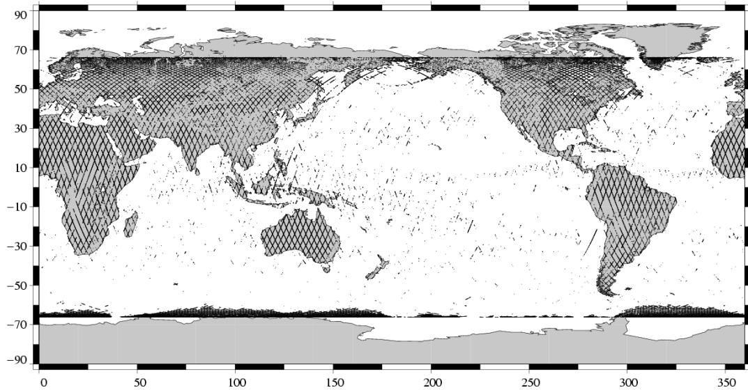
Edited measurements Jason-1 Cycle 125 (28/05/2005 / 07/06/2005)
