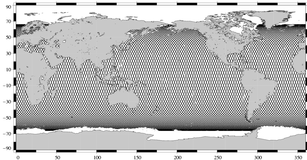
Valid data Jason-1 Cycle 125 (28/05/2005 / 07/06/2005)
