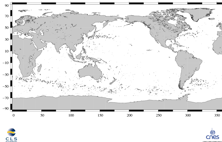
(SSH - MSS) differences greater than 30 cm Jason / Cycle 125
