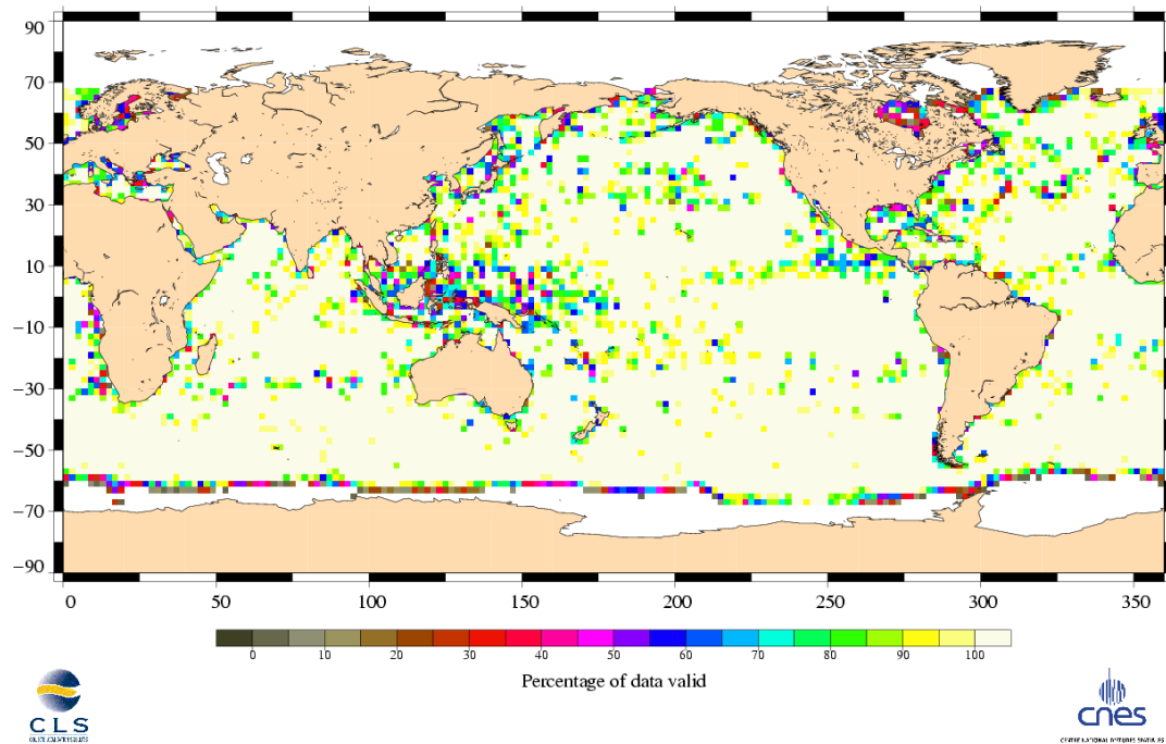
Percentage of valid data relative to the nominal pass Jason-1 Cycle 129 (07/07/2005 / 17/07/2005)
