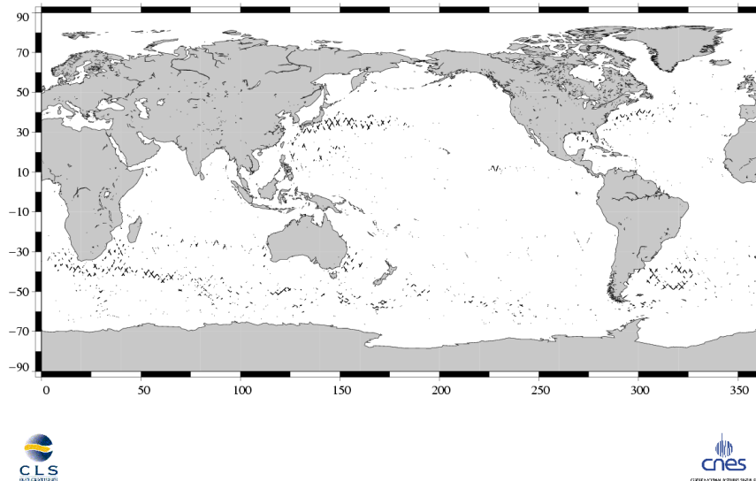
(SSH - MSS) differences greater than 30 cm Jason / Cycle 129
