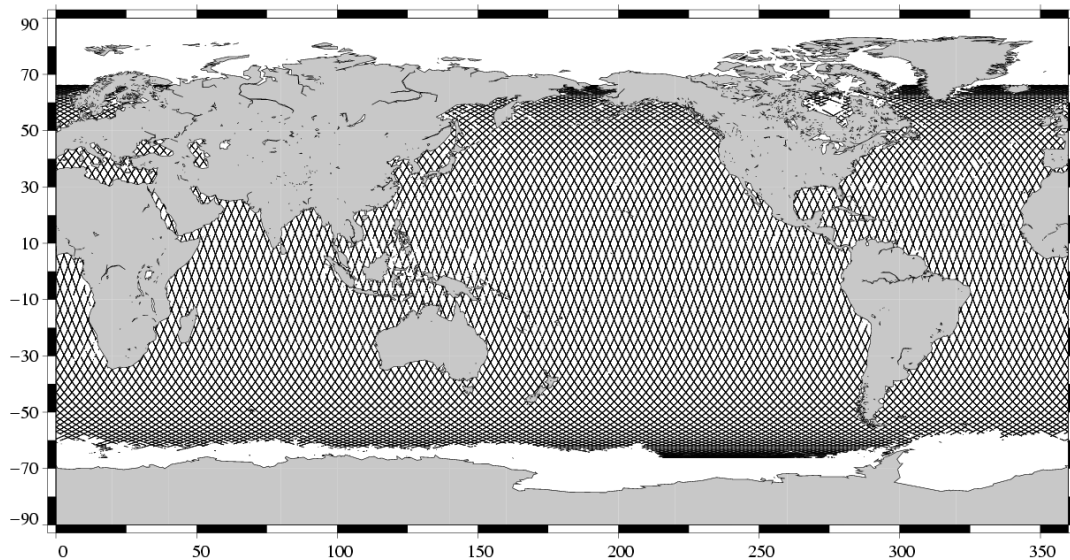
Valid data Jason-1 Cycle 129 (07/07/2005 / 17/07/2005)
