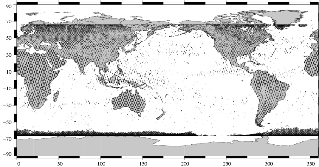
Edited measurements Jason-1 Cycle 129 (07/07/2005 / 17/07/2005)
