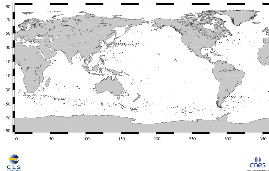
(SSH - MSS) differences greater than 30 cm Jason / Cycle 130
