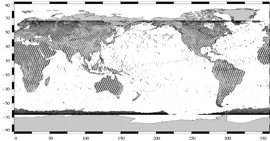
Edited measurements Jason-1 Cycle 130 (17/07/2005 / 27/07/2005)
