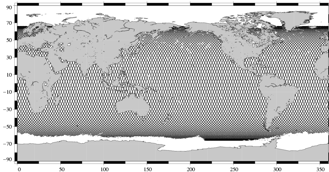
Valid data Jason-1 Cycle 130 (17/07/2005 / 27/07/2005)
