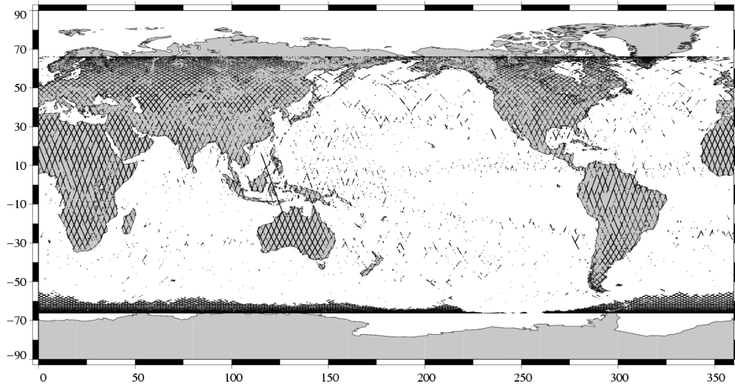
Edited measurements Jason-1 Cycle 131 (27/07/2005 / 06/08/2005)
