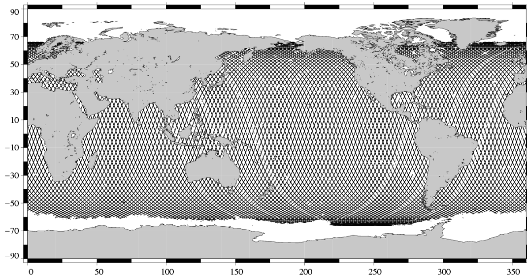
Valid data Jason-1 Cycle 131 (27/07/2005 / 06/08/2005)
