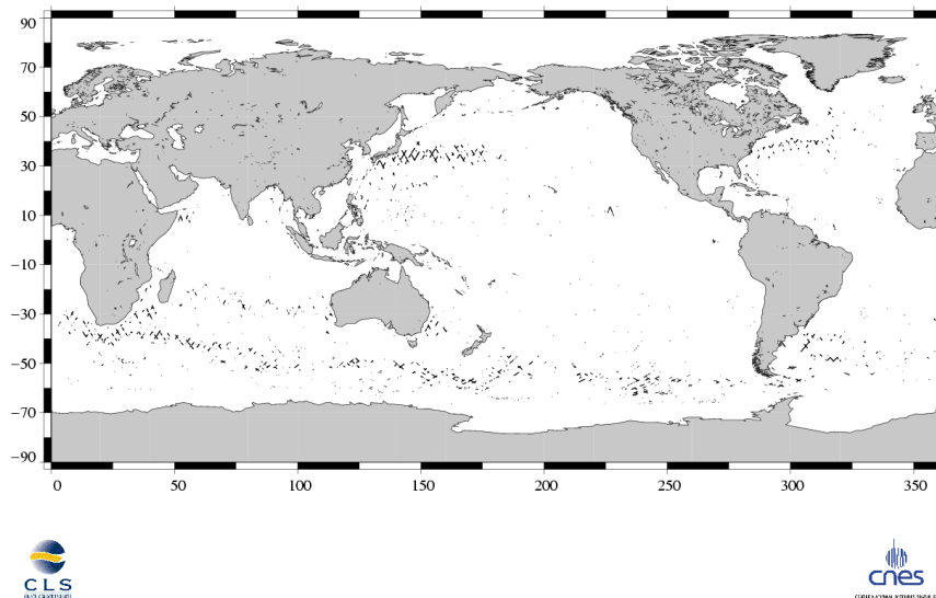
(SSH – MSS) differences greater than 30 cm Jason / Cycle 131
