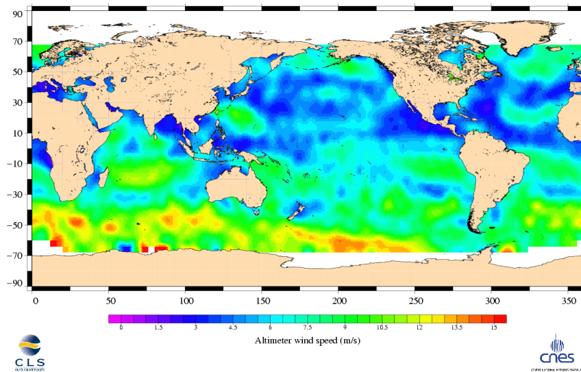
Jason-1 Cycle 134 25/08/2005 – 04/09/2005
