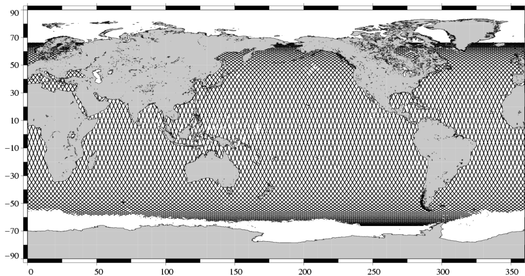
Valid data Jason-1 Cycle 139 (14/10/2005 / 24/10/2005)
