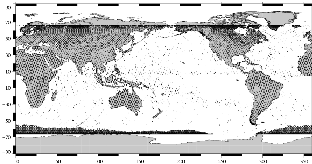
Edited measurements Jason-1 Cycle 141 (03/11/2005 / 13/11/2005)
