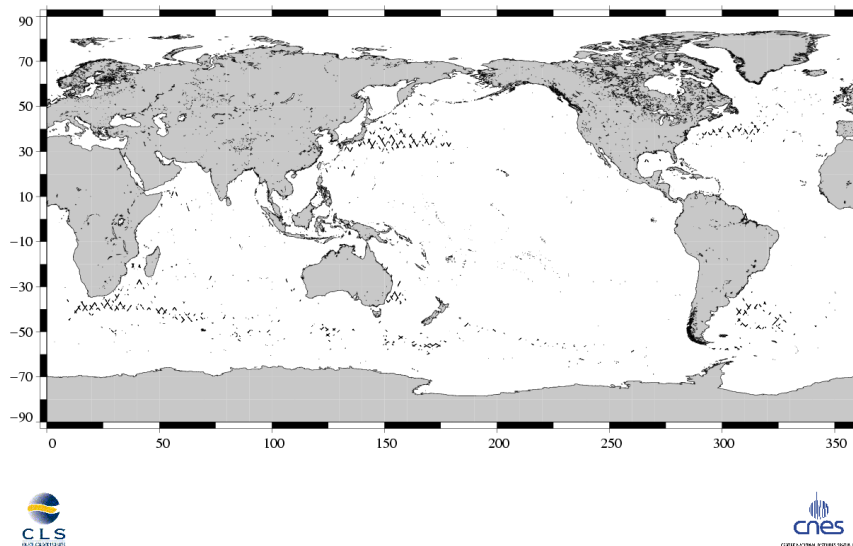
(SSH – MSS) differences greater than 30 cm Jason / Cycle 141
