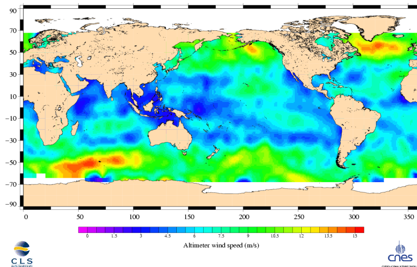
Jason-1 Cycle 141 03/11/2005 - 13/11/2005
