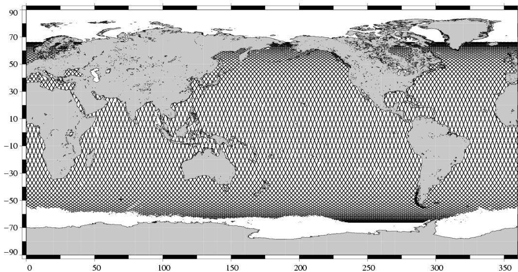
Valid data Jason-1 Cycle 141 (03/11/2005 / 13/11/2005)
