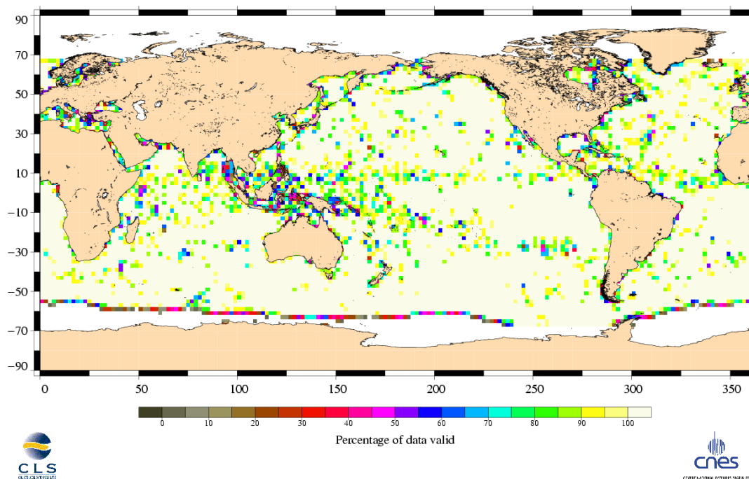
Percentage of valid data relative to the nominal pass Jason-1 Cycle 141 (03/11/2005 / 13/11/2005)
