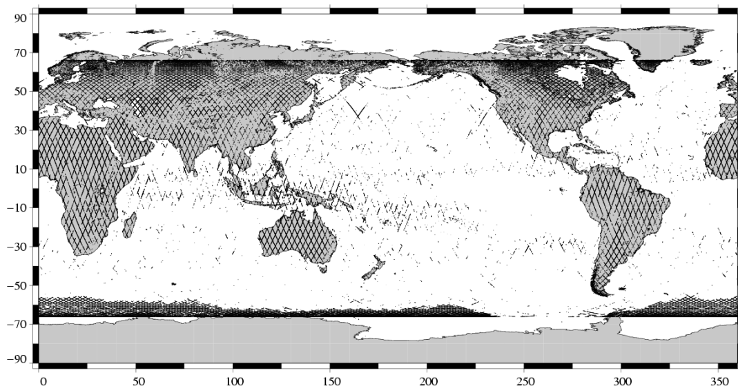
Edited measurements Jason-1 Cycle 142 (13/11/2005 / 23/11/2005)
