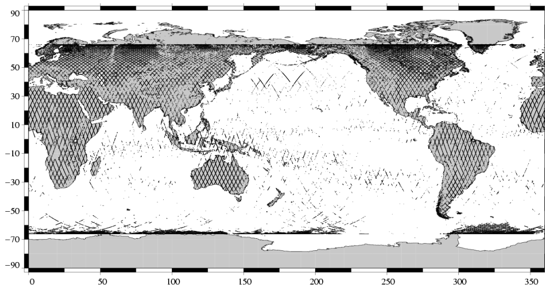
Edited measurements Jason-1 Cycle 146 (22/12/2005 / 01/01/2006)
