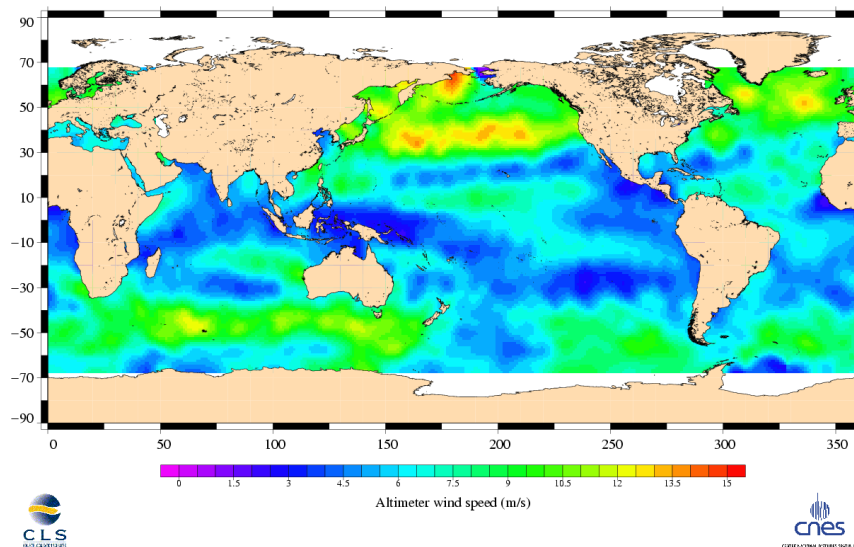
Jason-1 Cycle 146 22/12/2005 - 01/01/2006
