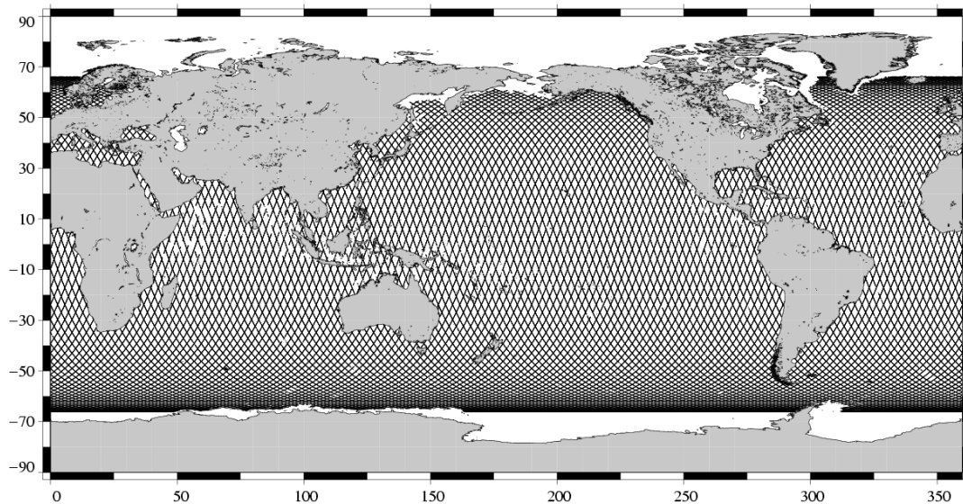
Valid data Jason-1 Cycle 157 (11/04/2006 / 20/04/2006)
