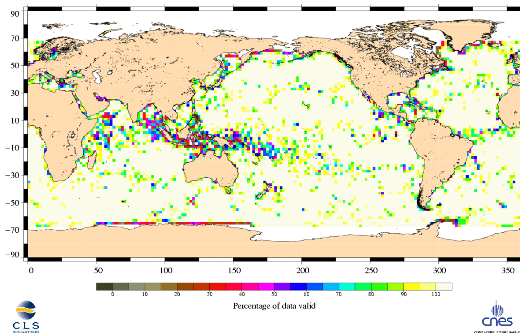
Percentage of valid data relative to the nominal pass Jason-1 Cycle 157 (11/04/2006 / 20/04/2006)
