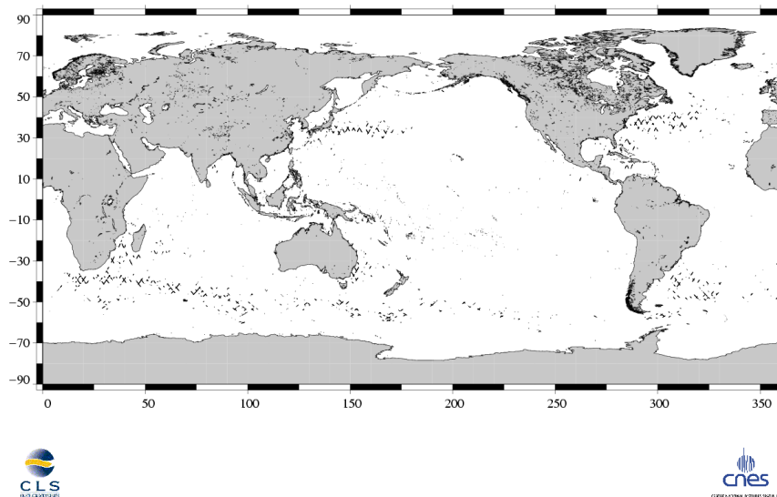
(SSH – MSS) differences greater than 30 cm Jason / Cycle 157
