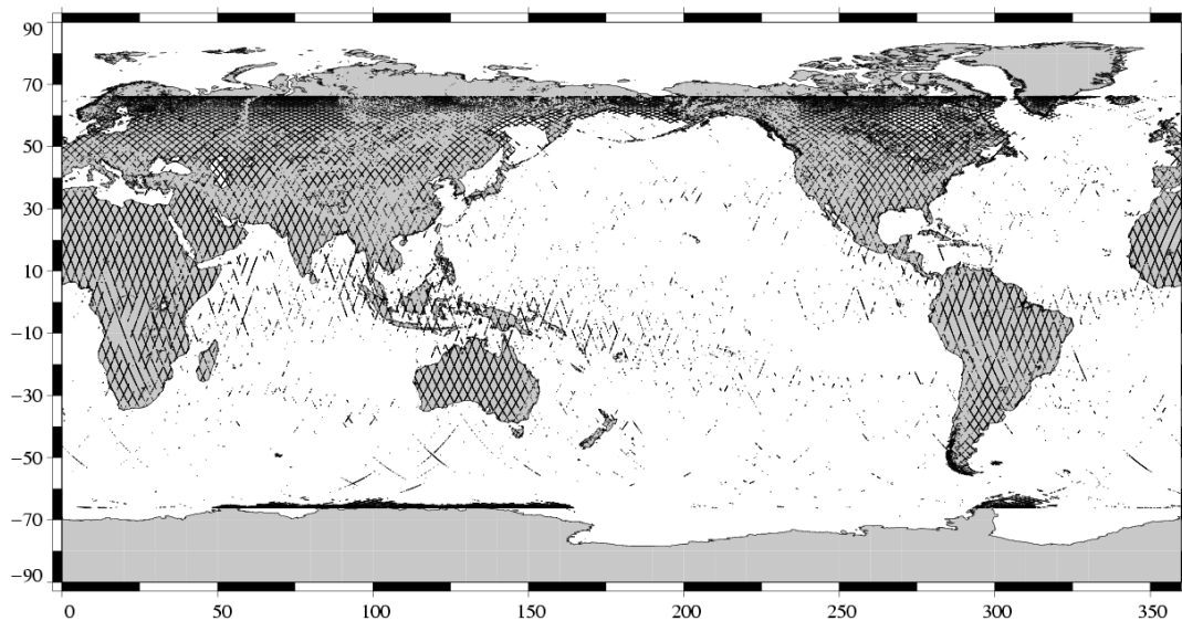
Edited measurements Jason-1 Cycle 157 (11/04/2006 / 20/04/2006)
