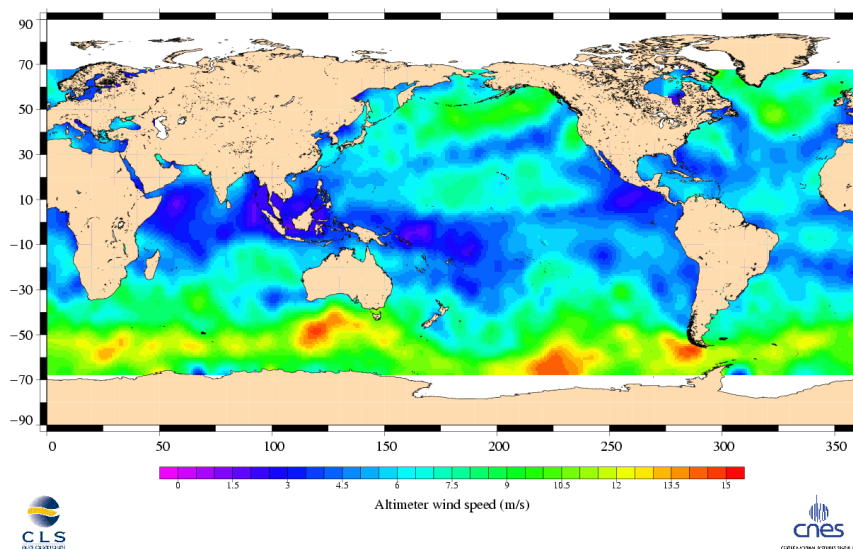
Jason-1 Cycle 159 30/04/2006 - 10/05/2006
