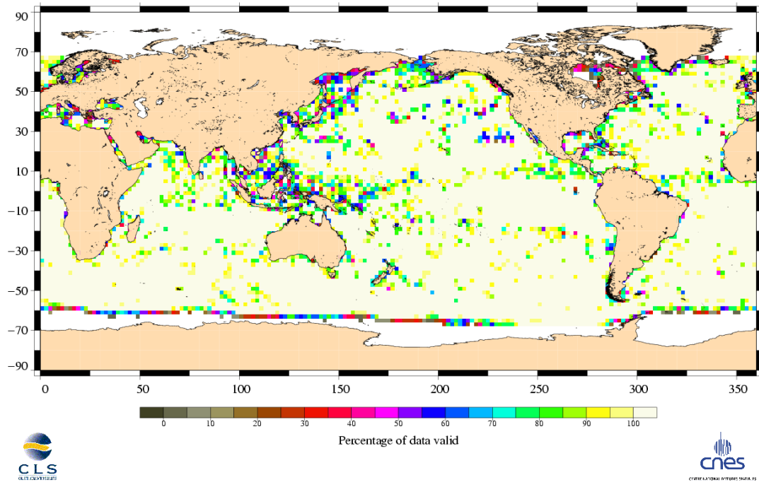
Percentage of valid data relative to the nominal pass Jason-1 Cycle 164 (19/06/2006 / 29/06/2006)
