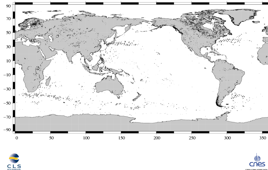
(SSH – MSS) differences greater than 30 cm Jason / Cycle 164
