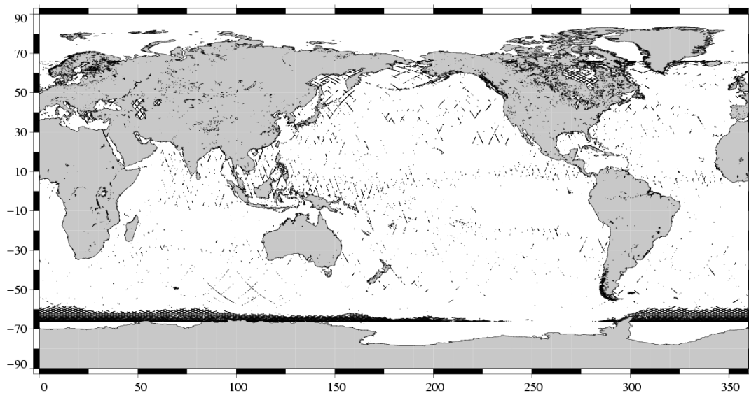
Edited measurements Jason-1 Cycle 164 (19/06/2006 / 29/06/2006)
