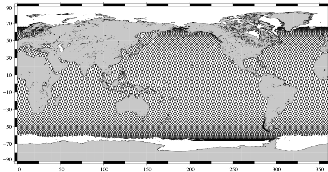
Valid data Jason-1 Cycle 164 (19/06/2006 / 29/06/2006)
