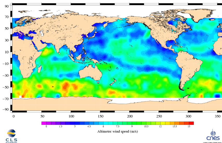
Jason-1 Cycle 164 19/06/2006 - 29/06/2006
