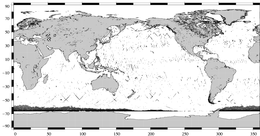
Edited measurements Jason-1 Cycle 165 (29/06/2006 / 09/07/2006)
