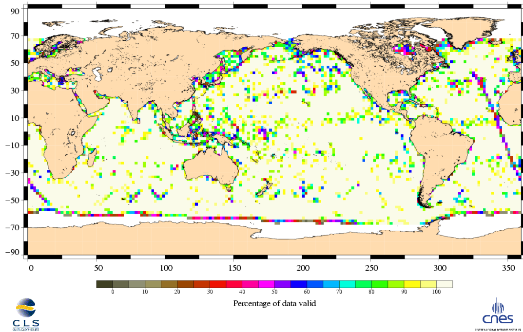
Percentage of valid data relative to the nominal pass Jason-1 Cycle 165 (29/06/2006 / 09/07/2006)
