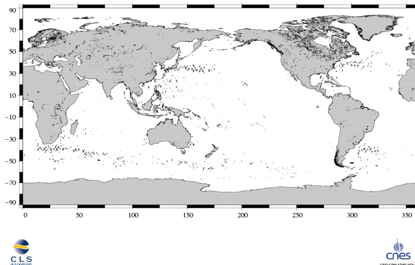
(SSH – MSS) differences greater than 30 cm Jason / Cycle 165
