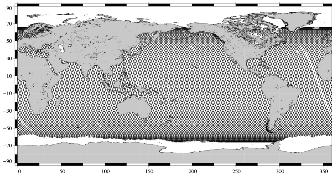
Valid data Jason-1 Cycle 165 (29/06/2006 / 09/07/2006)
