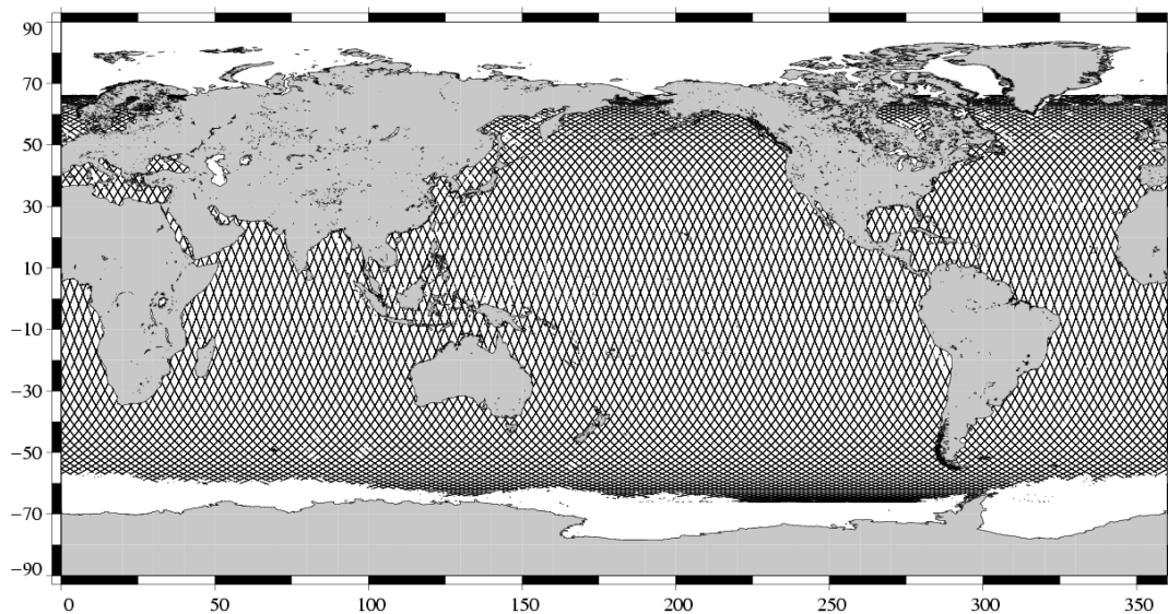
Valid data Jason-1 Cycle 167 (19/07/2006 / 29/07/2006)
