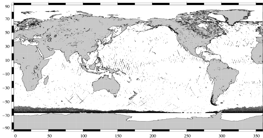
Edited measurements Jason-1 Cycle 167 (19/07/2006 / 29/07/2006)
