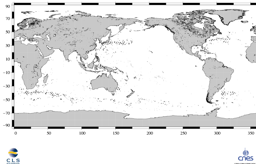
(SSH – MSS) differences greater than 30 cm Jason / Cycle 167
