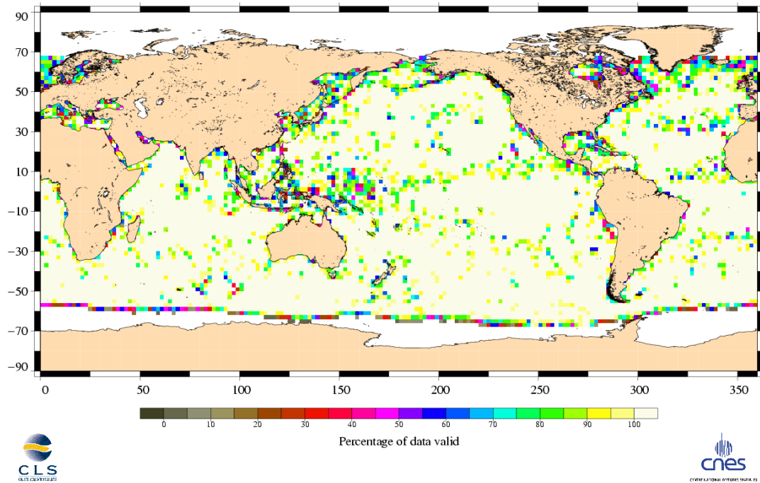
Percentage of valid data relative to the nominal pass Jason-1 Cycle 167 (19/07/2006 / 29/07/2006)
