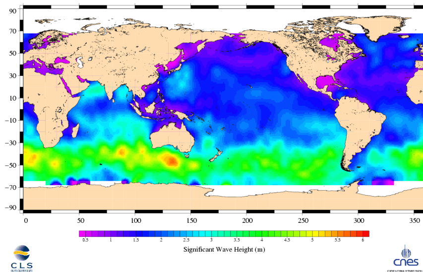
Jason-1 Cycle 169 08/08/2006 - 17/08/2006
