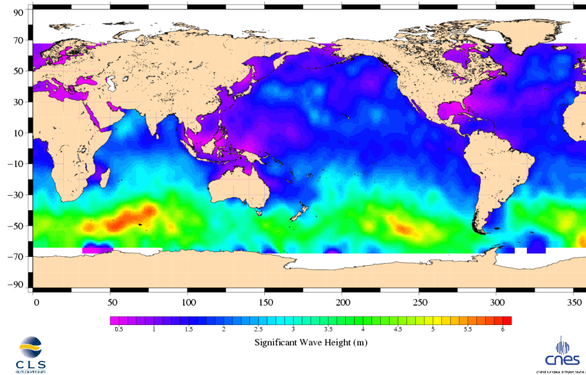
Jason-1 Cycle 170 17/08/2006 – 27/08/2006
