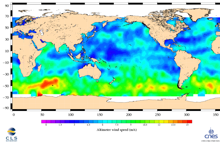
Jason-1 Cycle 170 17/08/2006 – 27/08/2006
